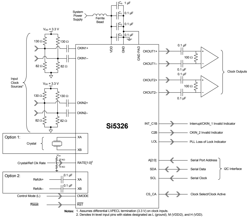
Figure 2. Si5326 Typical Application Circuit (I 2 C Control Mode)
