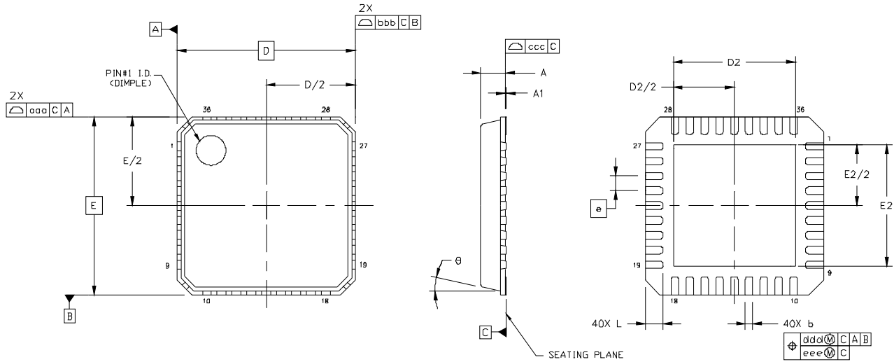
Figure 4. 36-Pin Quad Flat No-lead (QFN)
