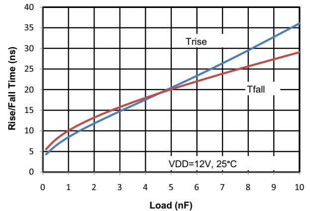
Figure 24. Rise/Fall Time vs. Load
