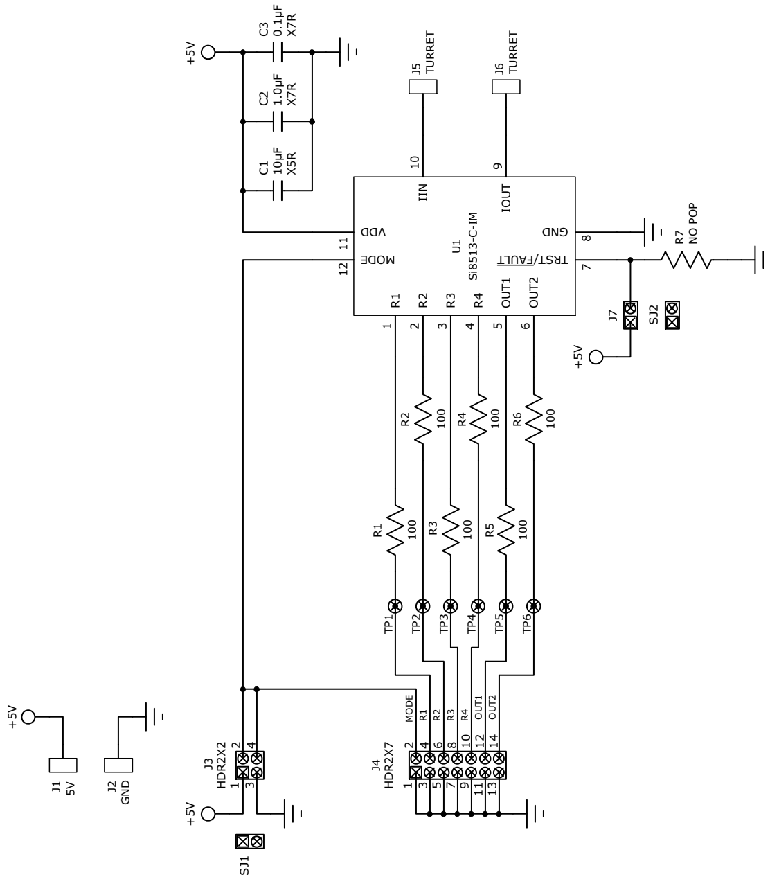
Figure 11. Si85xx Target Board Schematic (1 kV, 20 Amp Target Board)
