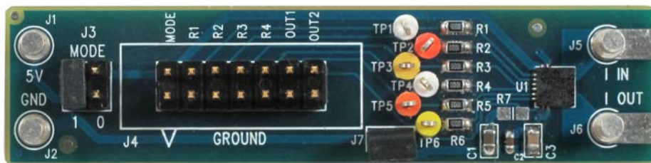
Figure 3. Si85xx20AQN-TB Overview (1 kV, 20 Amp Target Board)
