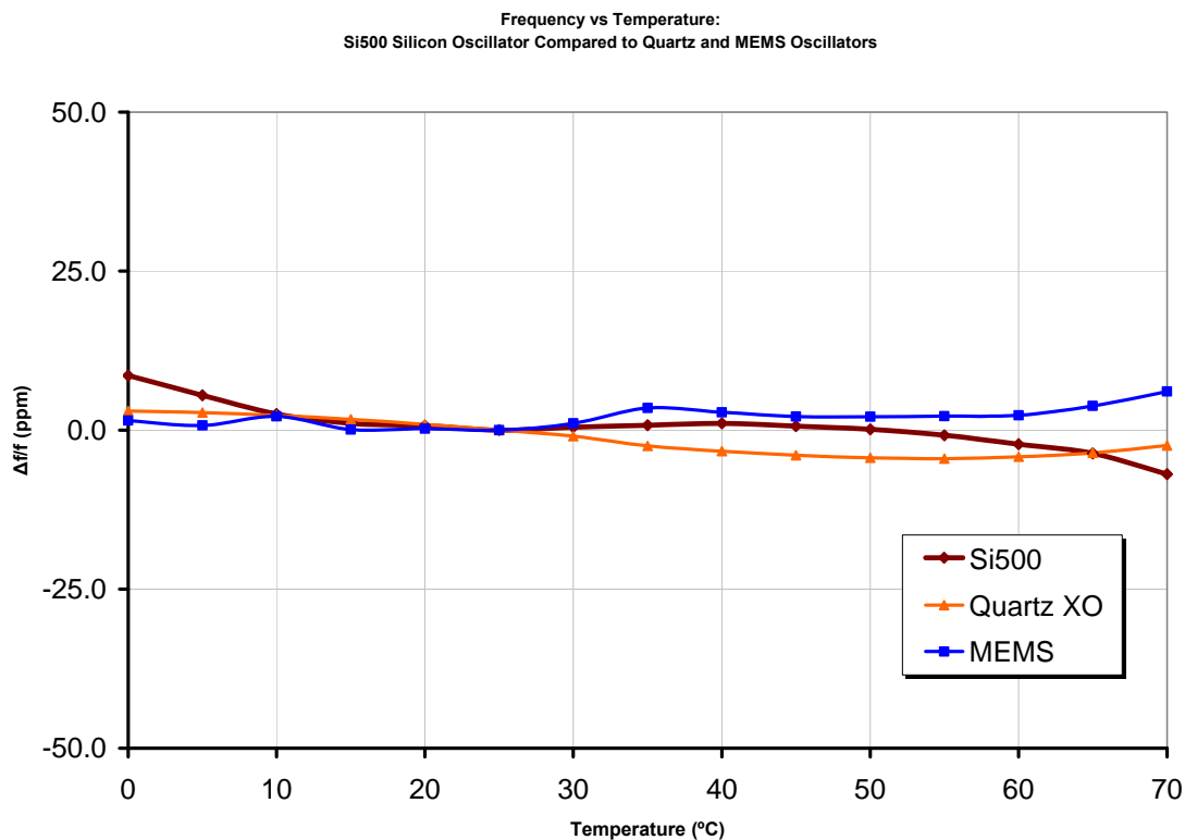
Figure 5 —Temperature Stability Comparison
