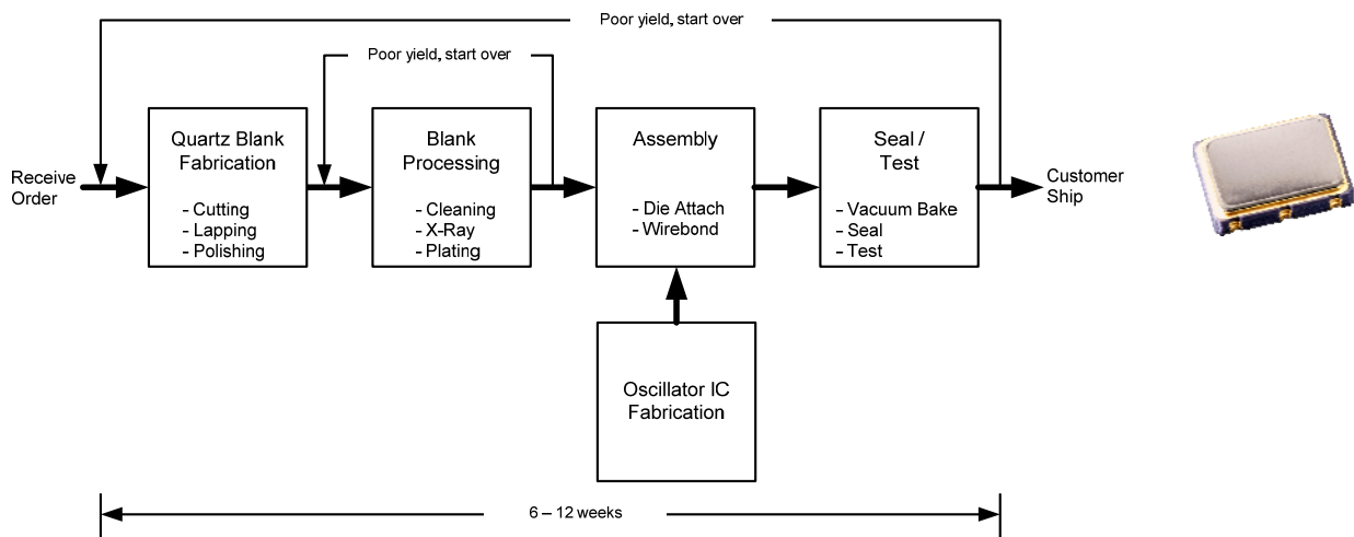
Figure 1 — Quartz Oscillator Manufacturing Flow
