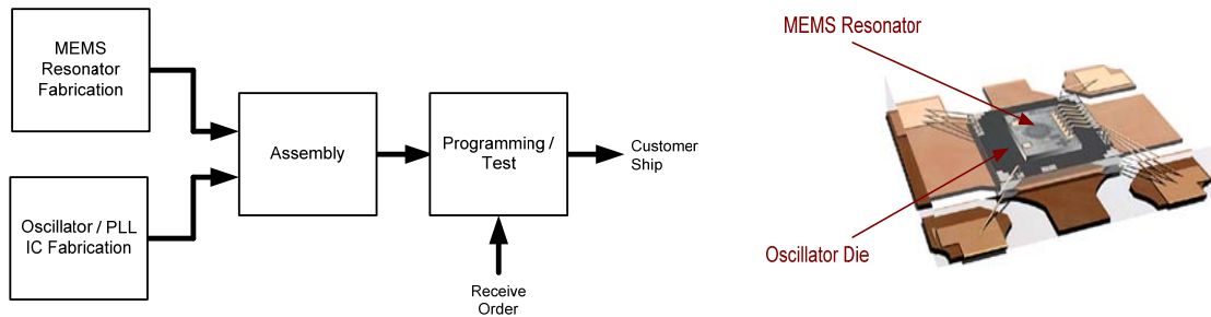
Figure 2 — MEMS Oscillator Manufacturing Flow
