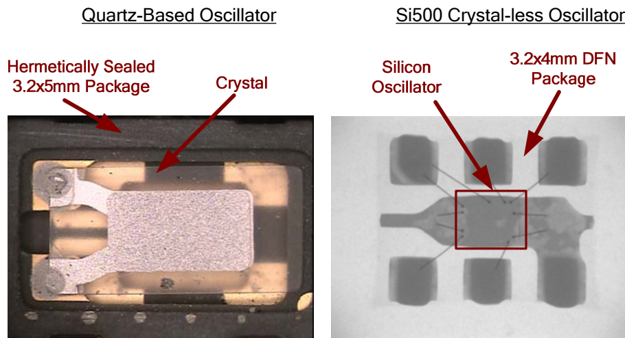
Figure 7 — Si500 vs. Quartz XO Packaging Comparison
