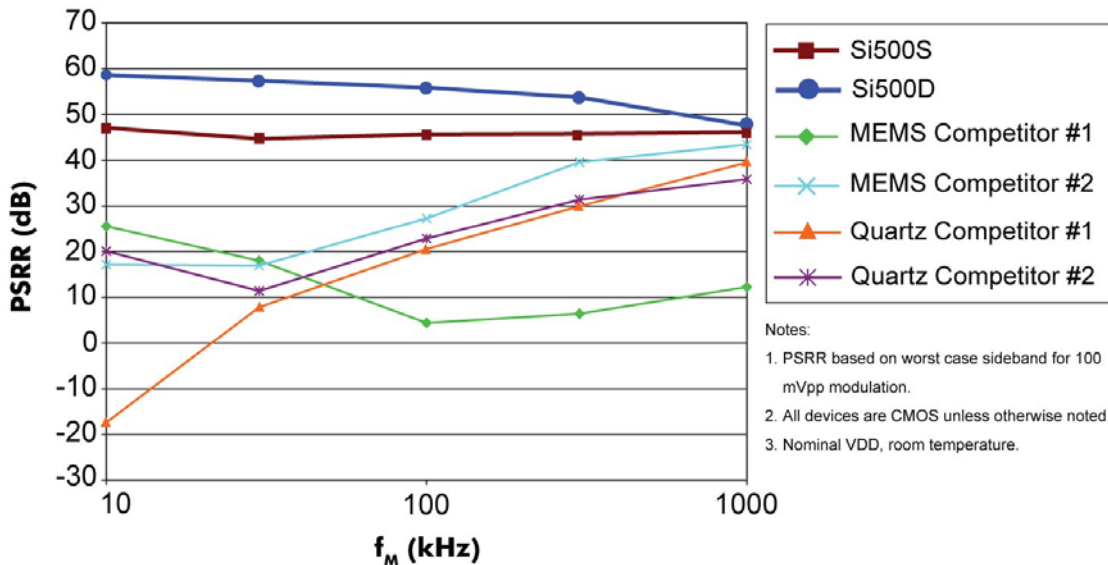
Figure 8 — PSRR Comparison
