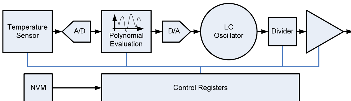
Figure 4 — Si500 Silicon Oscillator Block Diagram
