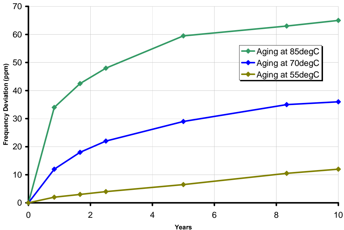
Figure 6 —Estimated Aging for Si500 Silicon Oscillator at 55, 70, and 85 °C
