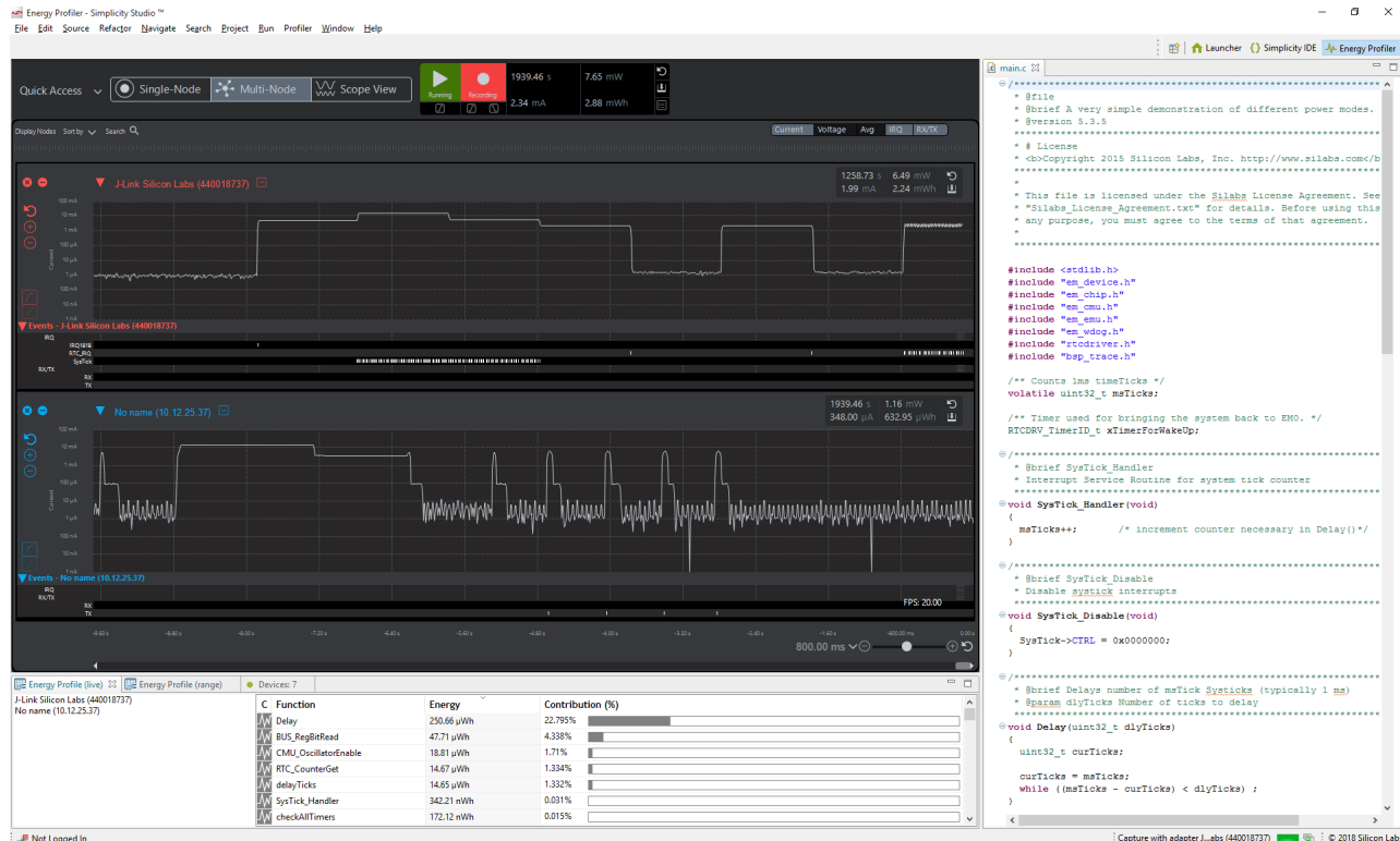
Figure 6.1. Energy Profiler
