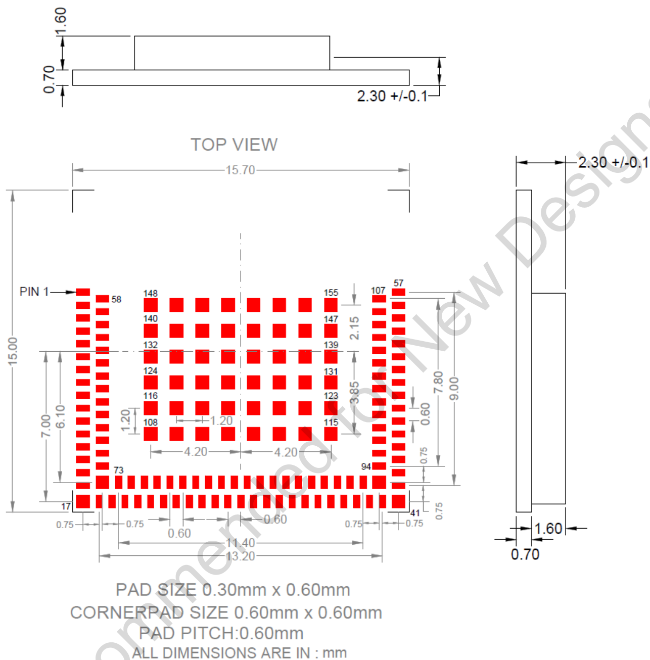
Figure 45. Package Outline
