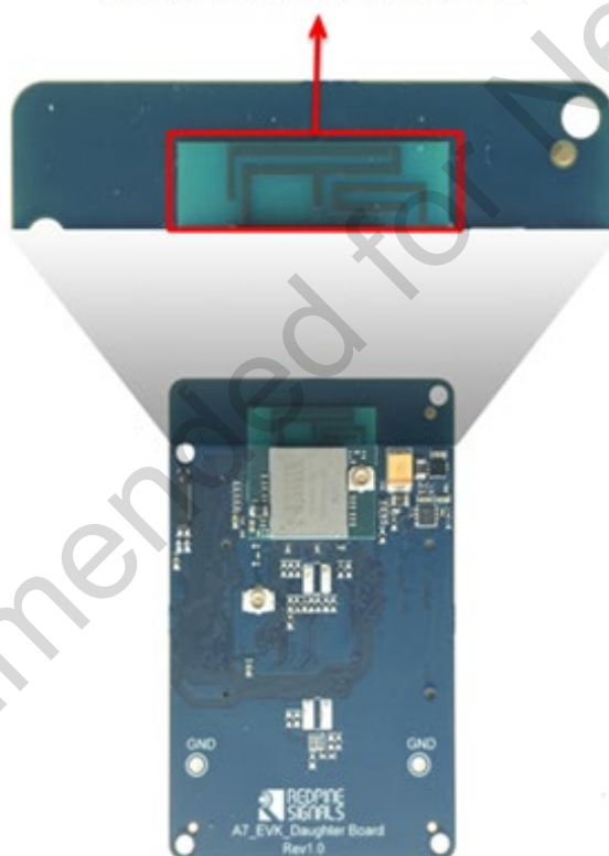
Figure 18. PCB Antenna Guidelines
