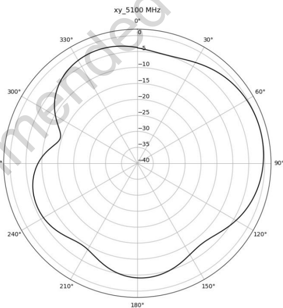
Figure 35. 2D Gain Plot for XY at 5.1 GHz
