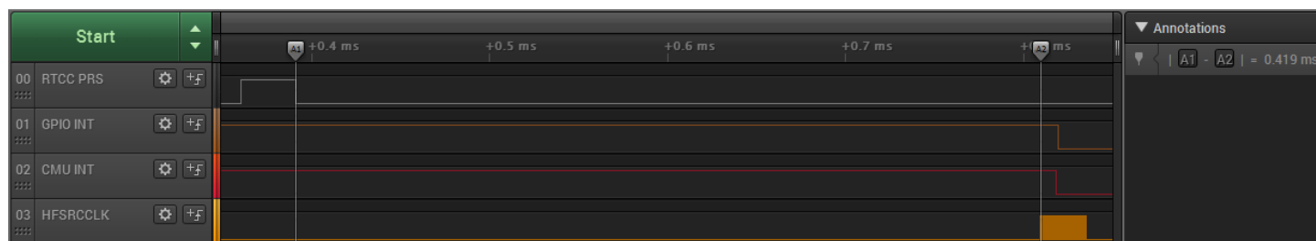
Figure 5.2. Automatic HFXO Start with Normal Start-up Time
