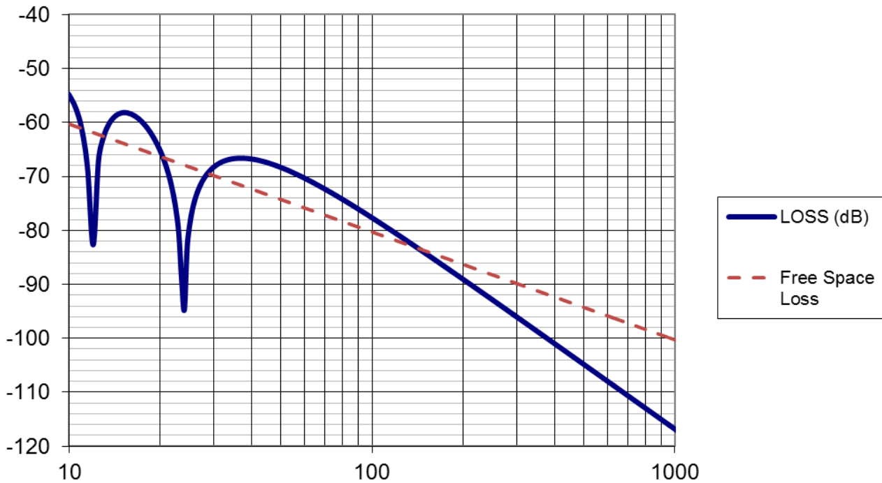
Figure 9: RF path loss in an open field with antennas 1.2 meters above ground
