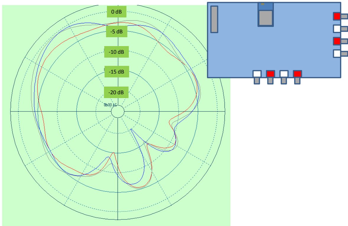
Figure 8: Radiation pattern of WT32i
