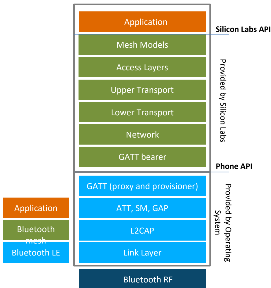
Figure 4-1: Bluetooth Stacks and Application Architecture on Smartphones
