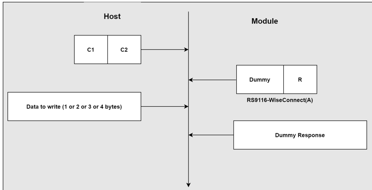
Figure 15: Register Write
