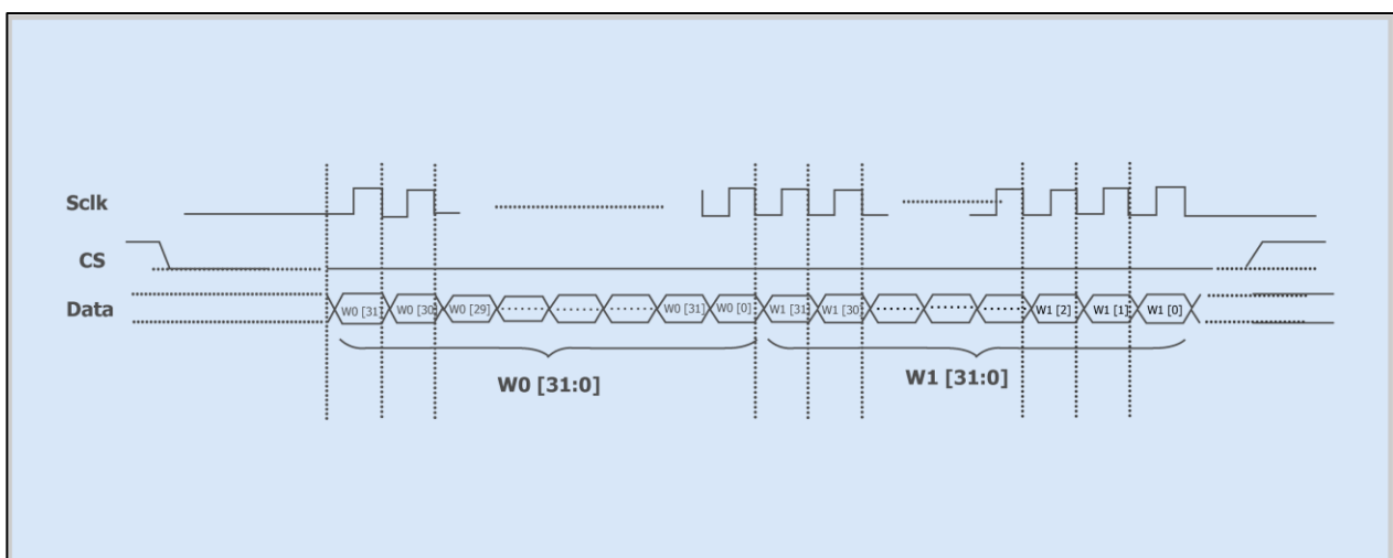
Figure 6 32-bit Mode
