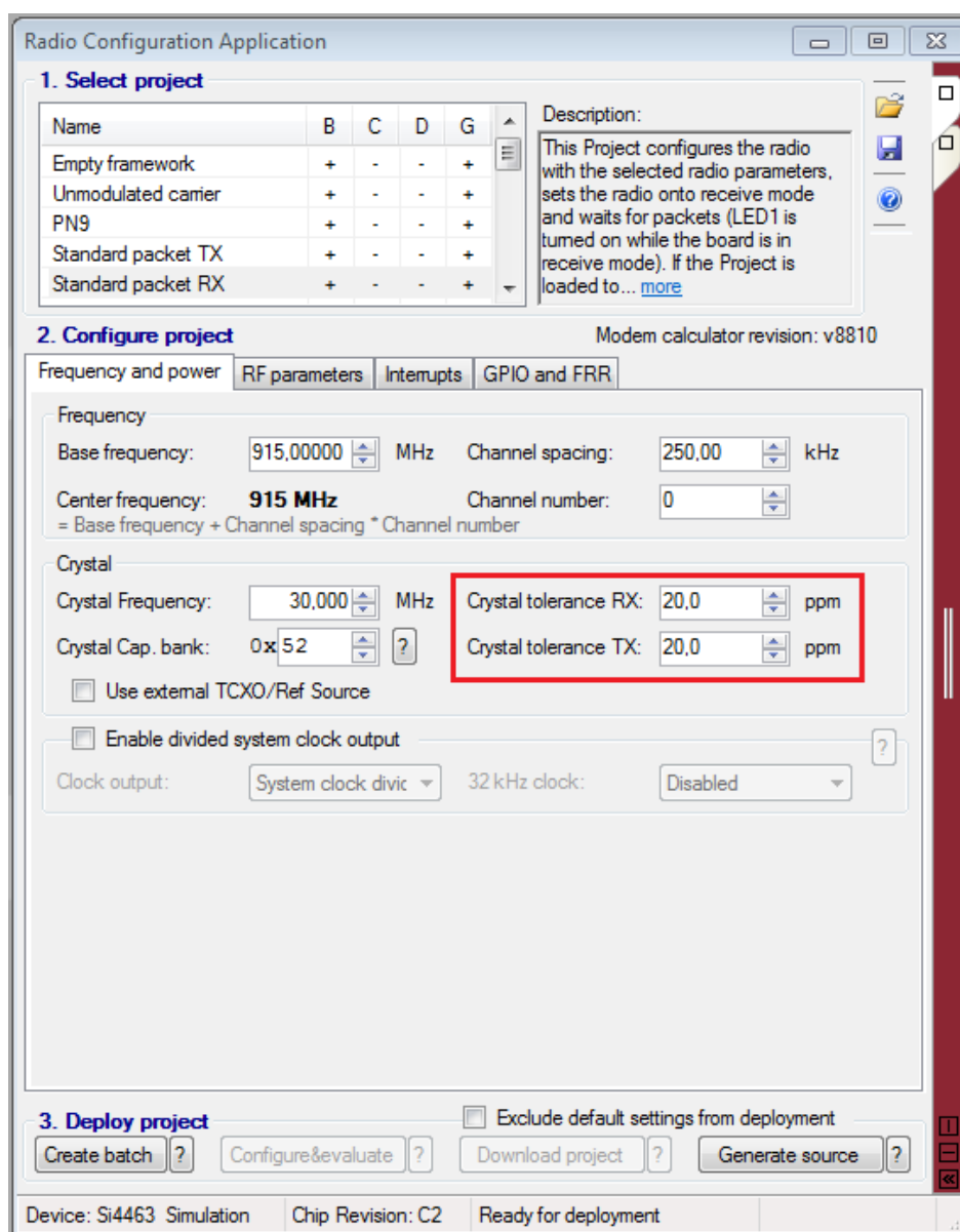
Figure 5. WDS Crystal Tolerance
