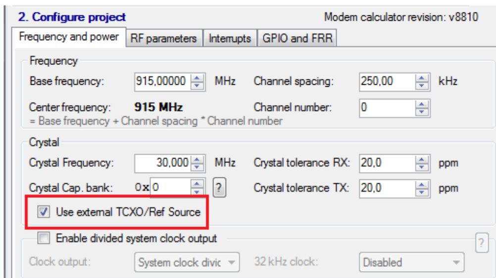
Figure 6. WDS setting for TCXO
