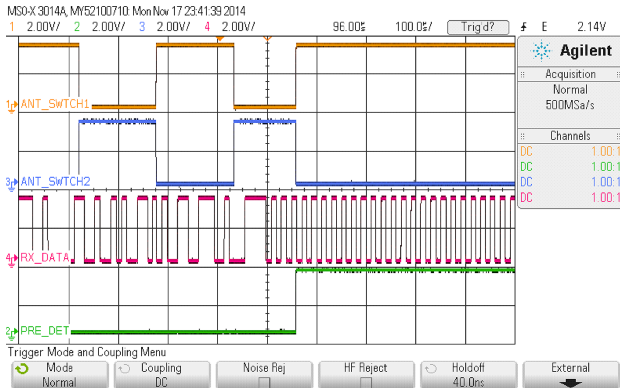
Figure 23. RX_DATA, PRE_DET, and Antenna Diversity Control Signals in Diversity Mode (Alternate Timing)
