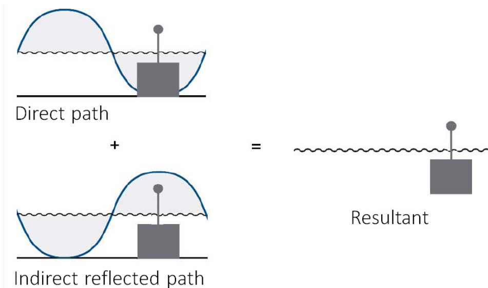
Figure 3. Worst Case RF Fading Effect from Phase Shifts Caused by Multipath
