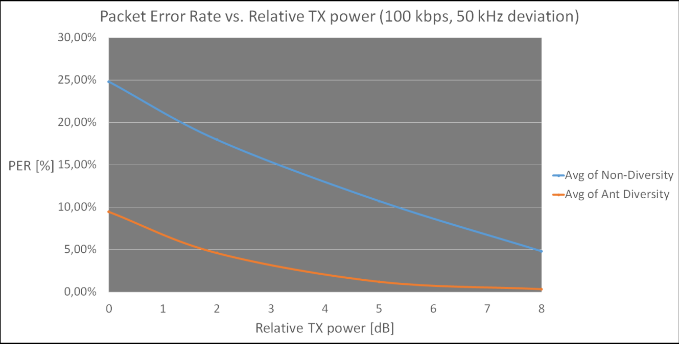
Figure 15. Packet Error Rate vs. Relative TX Power (Data Rate = 100 kbps)
