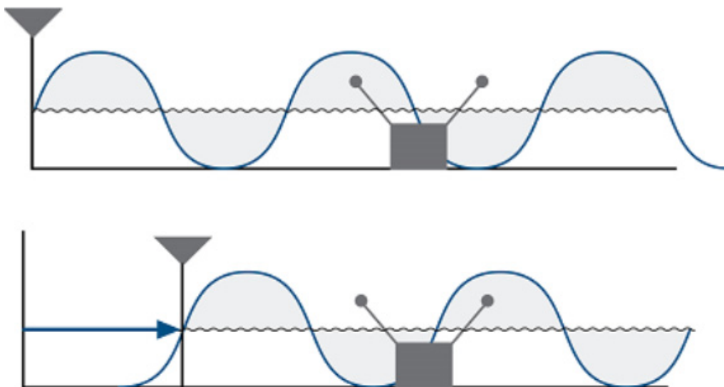
Figure 5. Combating RF Fading with Multiple Antennas
