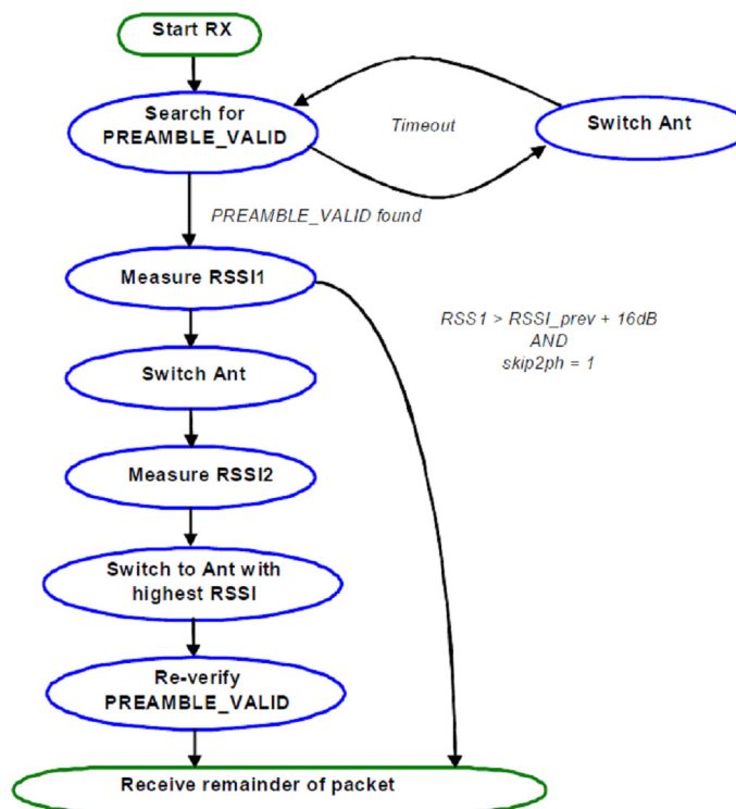
Figure 7. State Diagram of Antenna Diversity Algorithm
