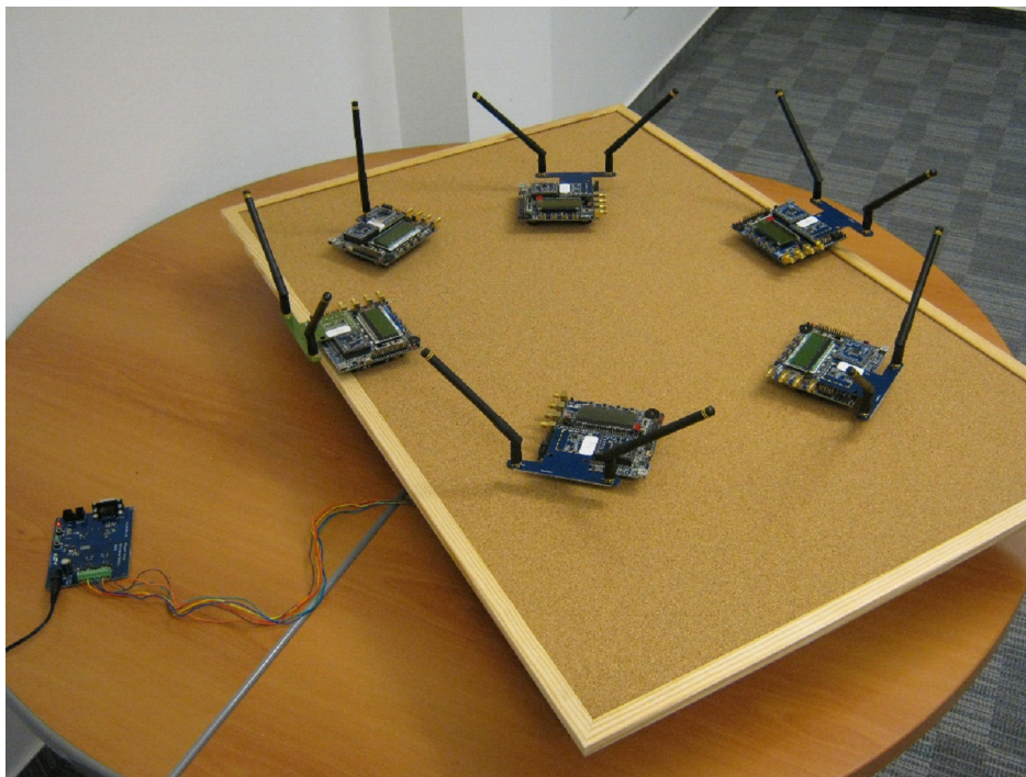
Figure 11. Measurement Setup with Turntable (Artificial Fading Simulator)
