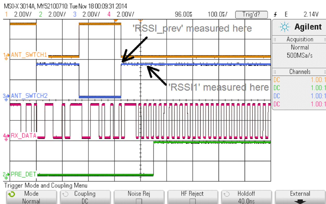
Figure 25. Skipping Alternate Antenna Evaluation
