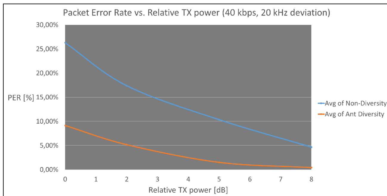
Figure 16. Packet Error Rate vs. Relative TX Power (Data Rate = 40 kbps)
