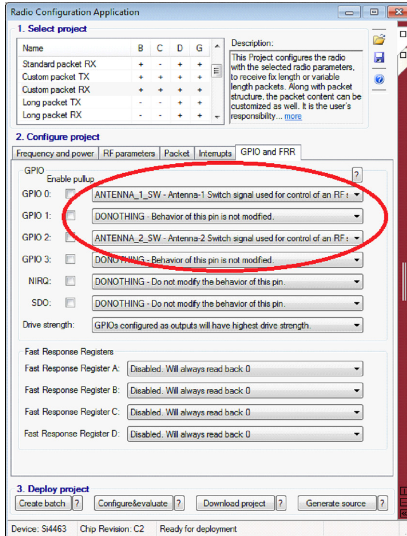
Figure 20. GPIO Settings in WDS
