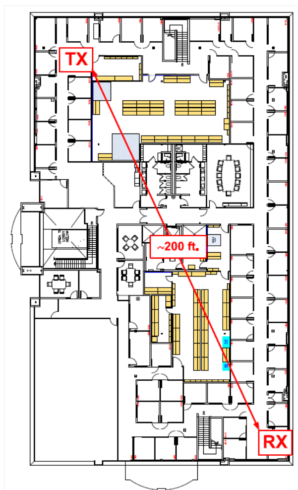
Figure 14. Plan View of the Indoor Office Environment for the Test, TX, and RX Locations Demonstrated
