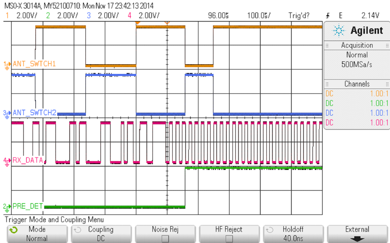
Figure 22. RX_DATA, PRE_DET, and Antenna Diversity Control Signals in Diversity Mode
