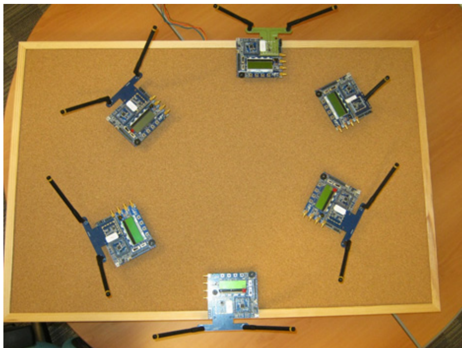
Figure 13. Arrangement of RF Test Boards on the Turntable
