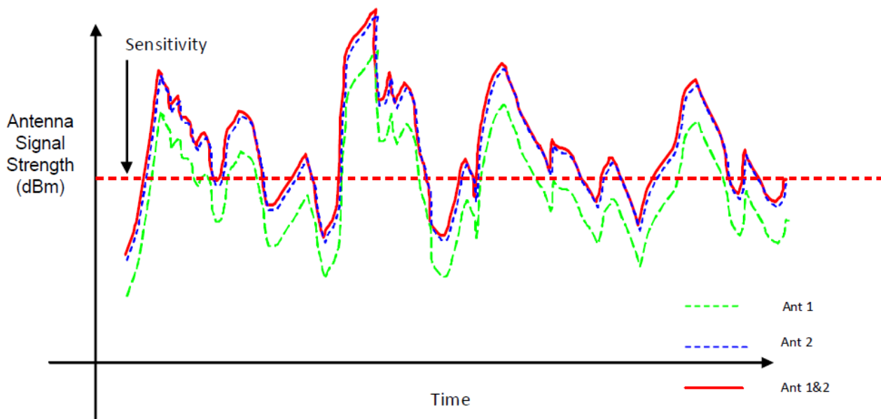
Figure 8. Antenna #1 and Antenna #2 with Correlated Signal Inputs
