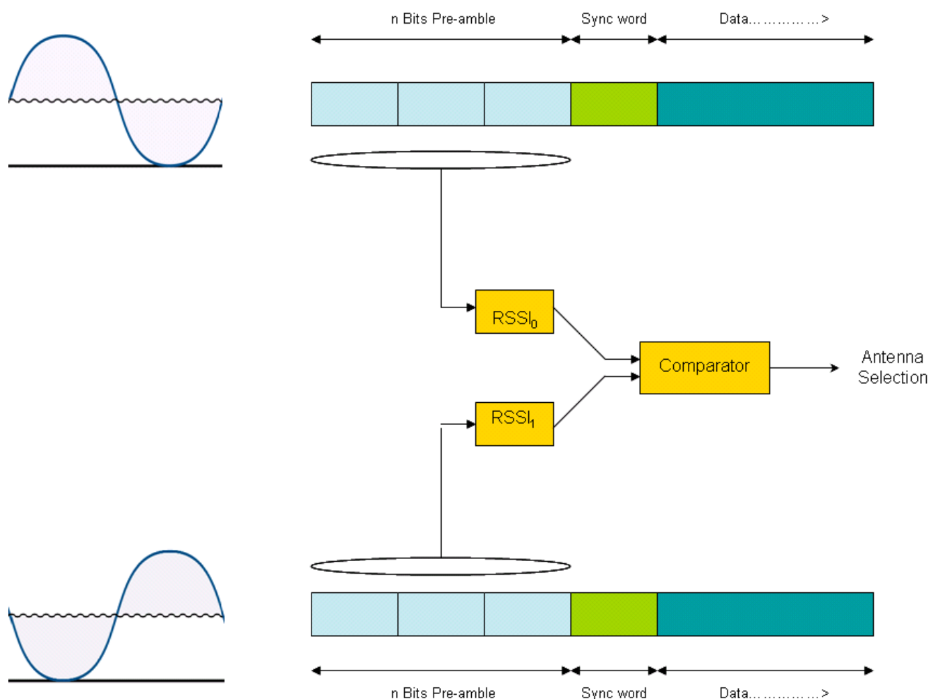
Figure 6. Measuring RSSI Levels to Qualify Antenna Selection
