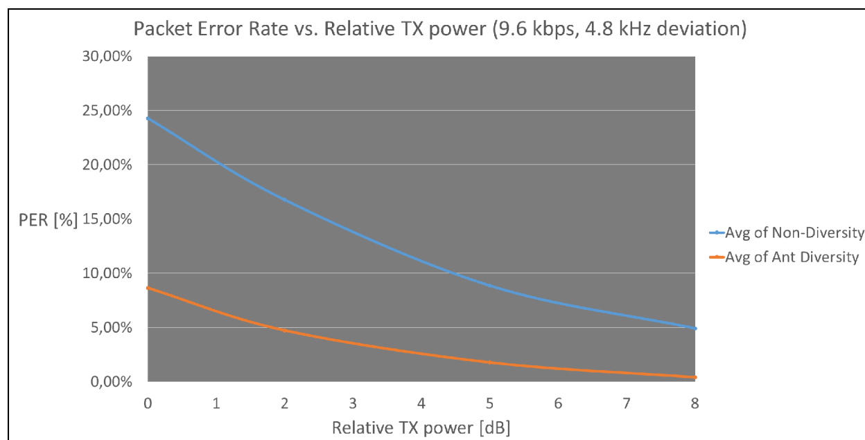
Figure 17. Packet Error Rate vs. Relative TX Power (Data Rate = 9.6 kbps)
