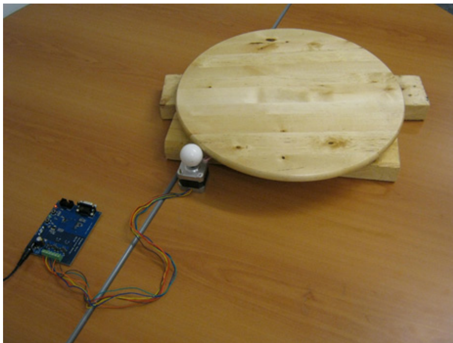
Figure 12. Rotating Motor
