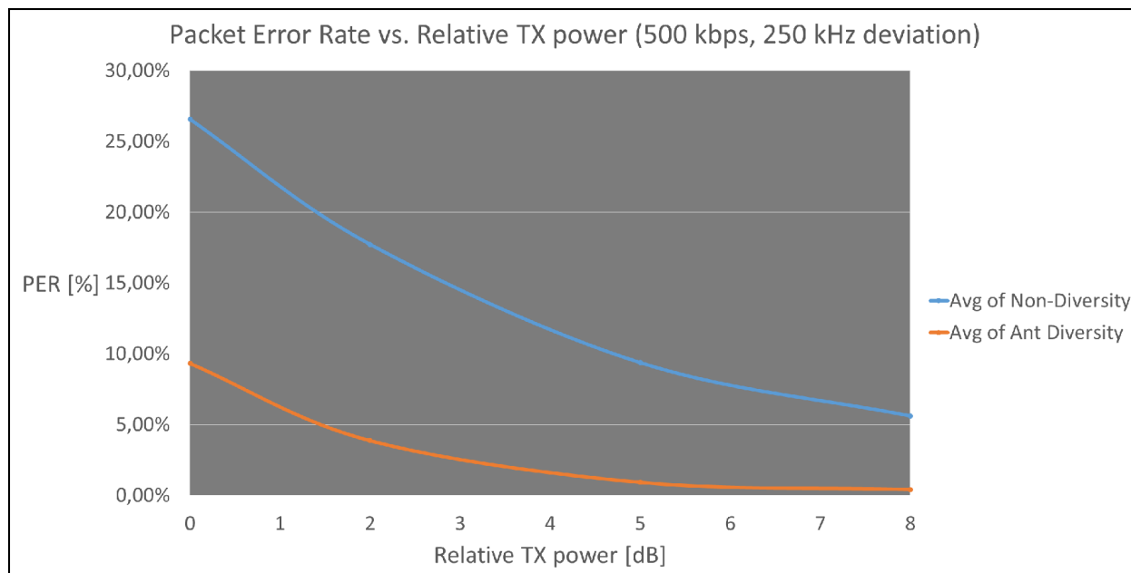
Figure 18. Packet Error Rate vs. Relative TX Power (Data Rate = 500 kbps)
