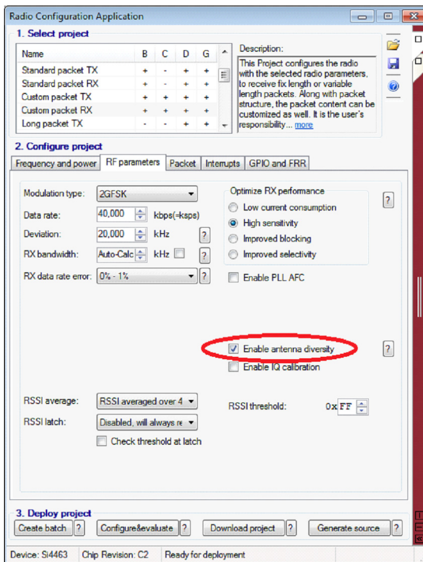
Figure 21. Antenna Diversity Enable
