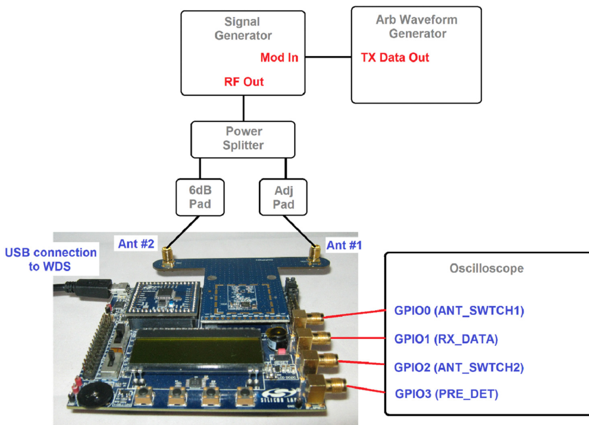
Figure 19. Lab Test Setup for Antenna Diversity
