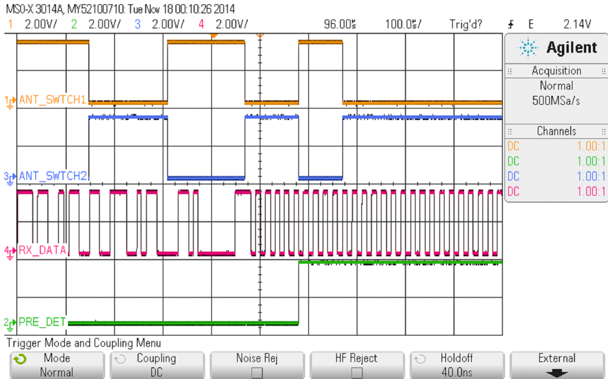
Figure 24. RX_DATA, PRE_DET, and Antenna Diversity Control Signals in Diversity Mode (Alternate RF Levels)
