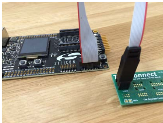
Figure 5.7. TC2030-CTX-20 Cable
