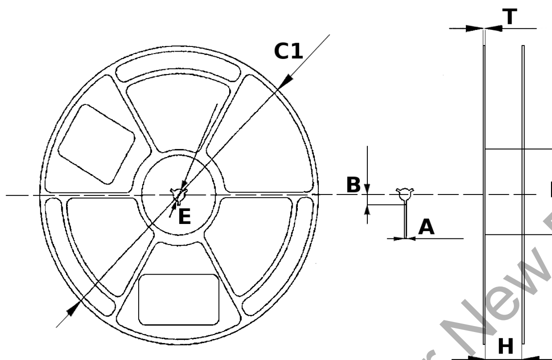
Figure 17 - Reel Specifications
