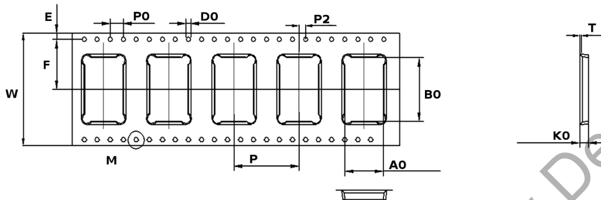
Figure 16 - Tape Specifications
