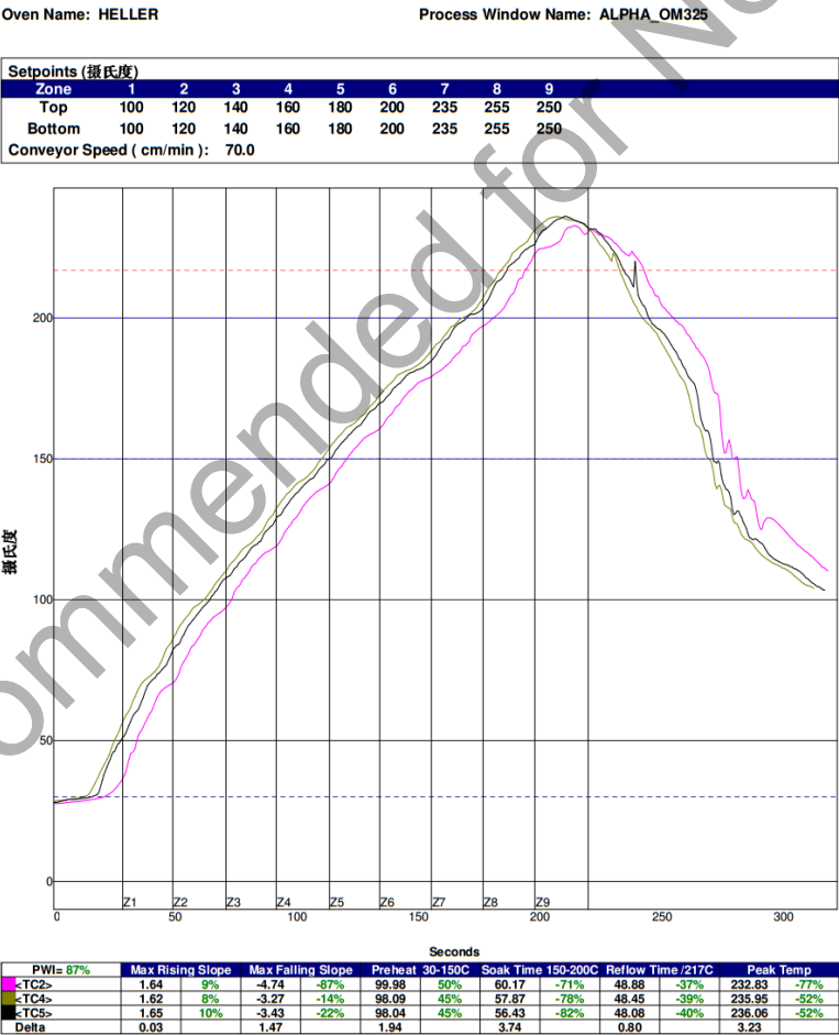
Figure 7 - Example solder reflow profile (AMW006-E03 evaluation board)
