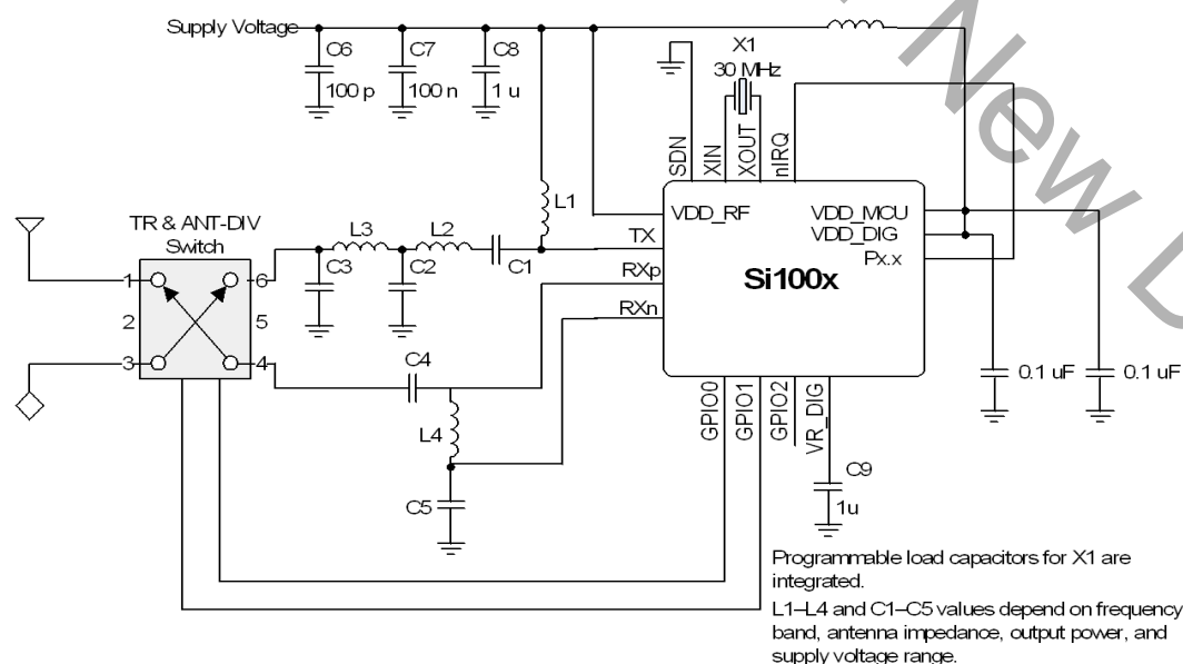
Figure 1.8. Si1000/1 Antenna Diversity Application Example
