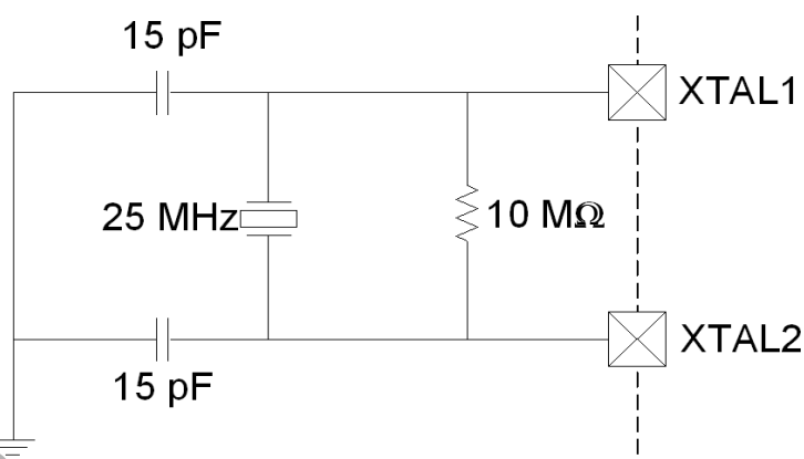
Figure 19.2. 25 MHz External Crystal Example
