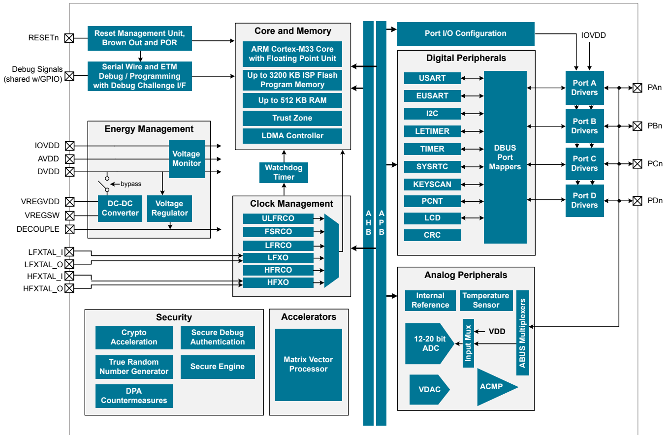
Figure 3.1. Detailed EFM32PG26 Block Diagram
