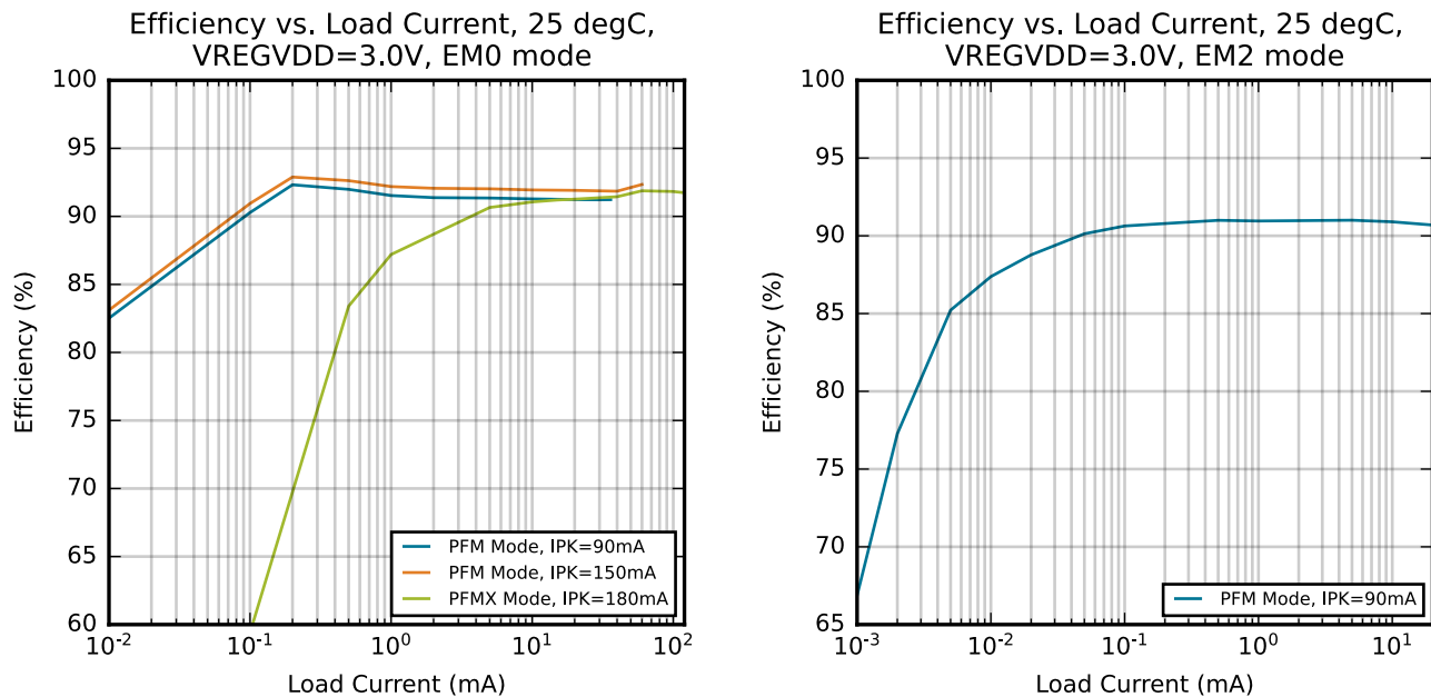
Figure 4.11. DC-DC Efficiency
