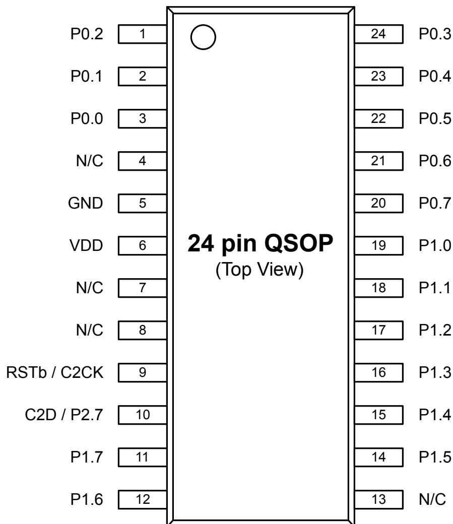
Figure 6.3. EFM8SB1x-QSOP24 Pinout
