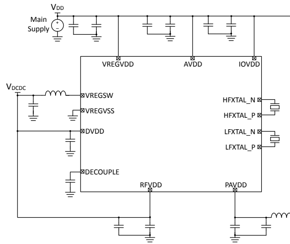
Figure 5.3. EFR32FG14 Typical Application Circuit: Configuration with DC-DC converter (PAVDD from VDD)
