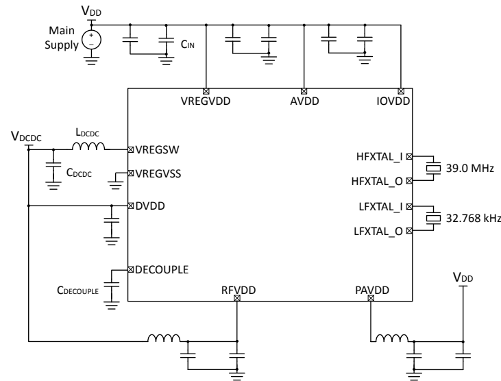
Figure 5.3. EFR32FG23L Typical Application Circuit: DCDC Configuration, PAVDD Powered Separately
