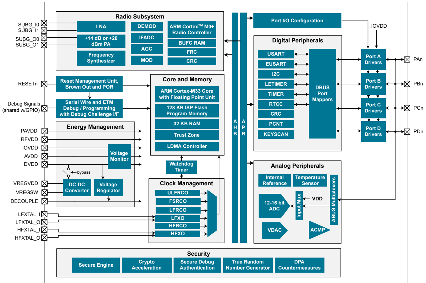
Figure 3.1. Detailed EFR32FG23L Block Diagram
