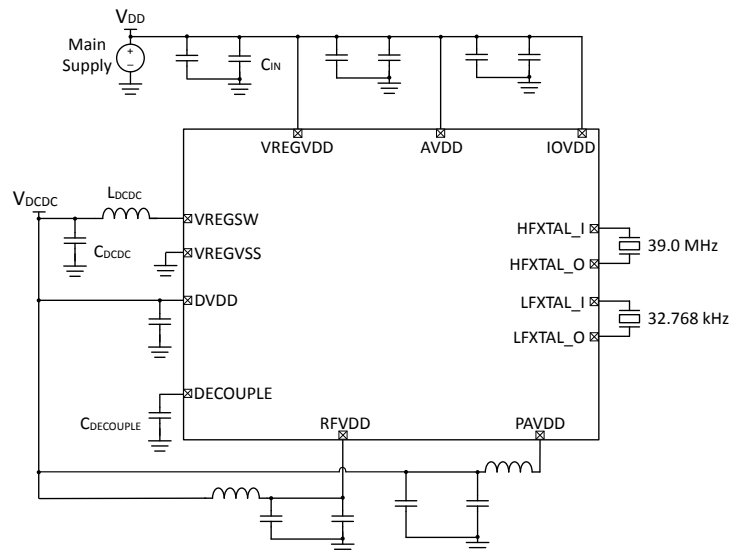
Figure 5.2. EFR32FG23L Typical Application Circuit: DCDC Configuration
