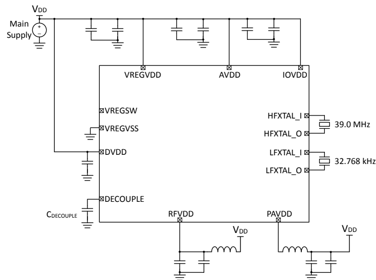
Figure 5.1. EFR32FG23L Typical Application Circuit: Direct Supply Configuration without DCDC
