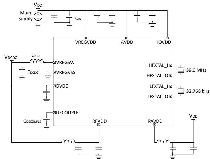
Figure 5.3. EFR32SG23 Typical Application Circuit: DCDC Configuration, PAVDD Powered Separately
