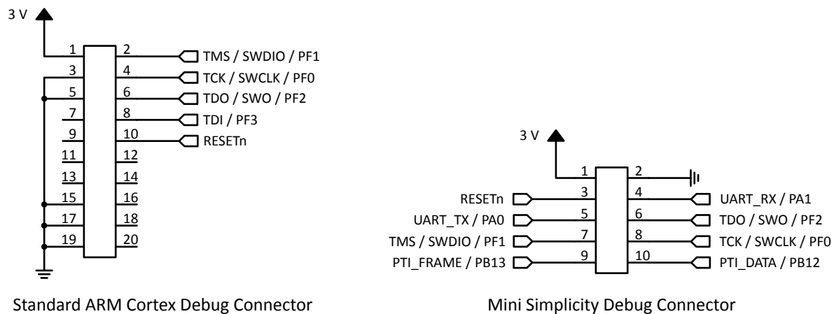
Figure 5.5. Common Debug Connections
