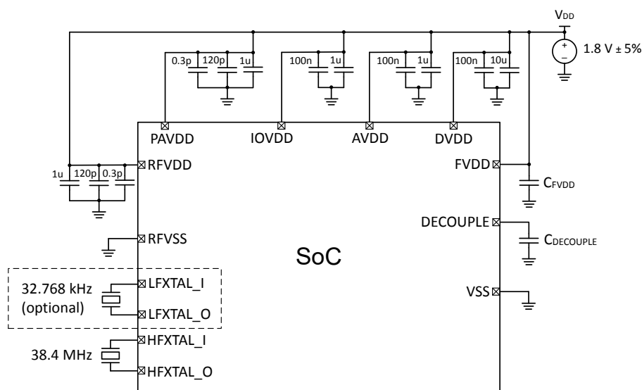
Figure 5.2. Single Supply (1.8 V \pm 5%)
