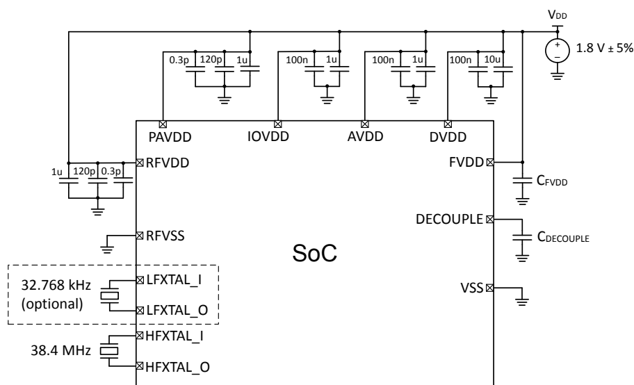
Figure 5.2. Single Supply ( 1.8 \text{ V} \pm 5\% )
