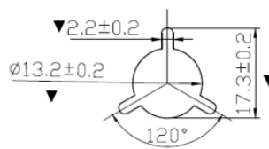
Figure 10.5. Central Axis Dimensions
