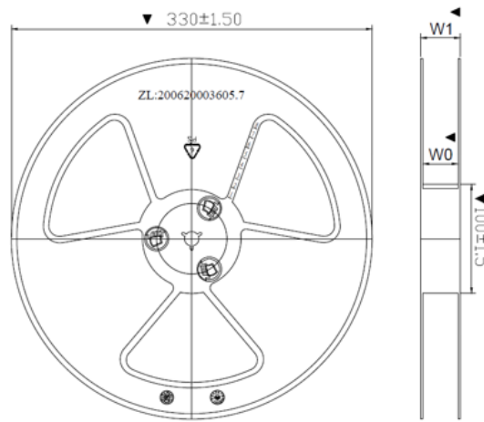
Figure 10.4. Reel Dimensions - Side View
