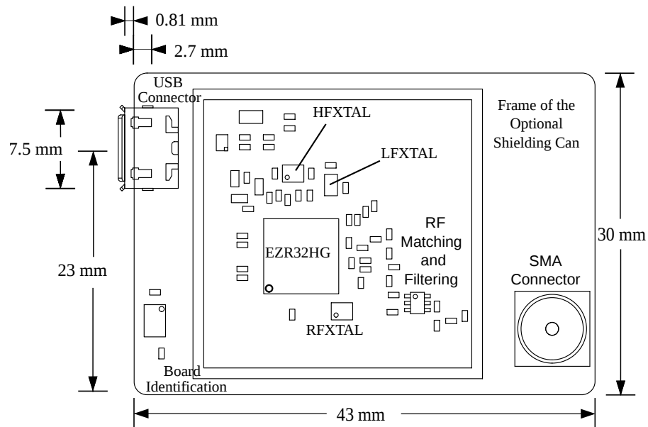
Figure 5.1. BRD4545A Top View
