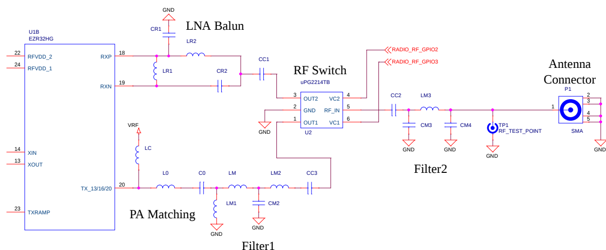
Figure 4.1. RF Section of the Schematic of the BRD4545A EZR32 Happy Gecko Radio Board
