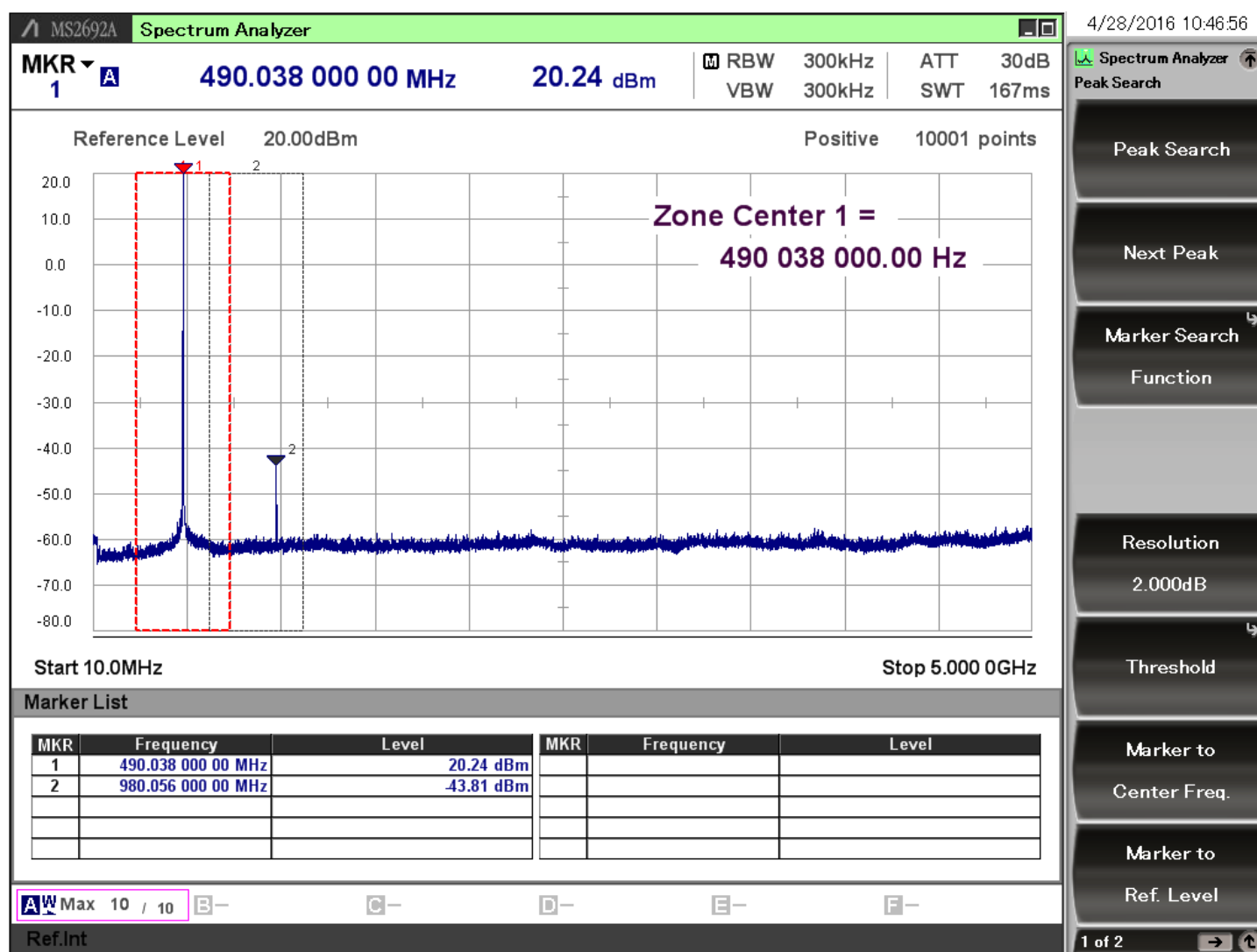
Figure 7.1. Typical Output Spectrum of the BRD4545A Radio Board
