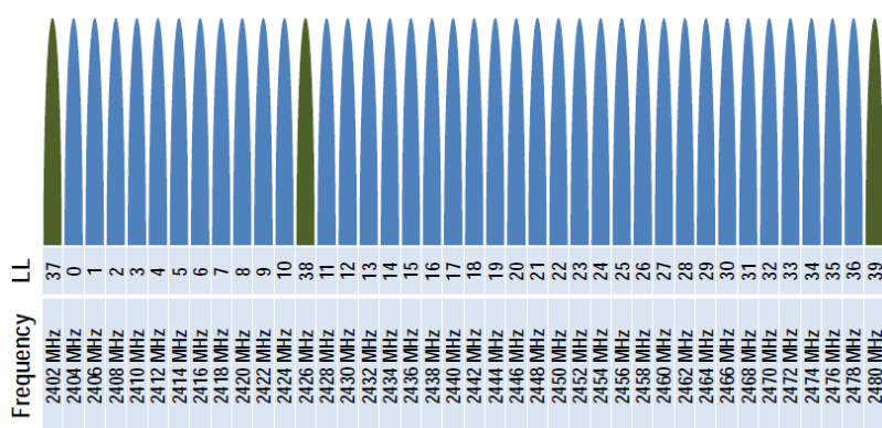
Figure: Link layer channels
