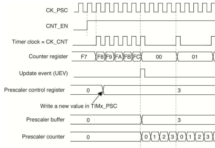
Figure 10.2. Counter Modes
