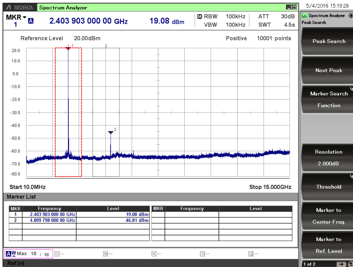
Figure 7.2. Typical Output Spectrum of the BRD4150B
