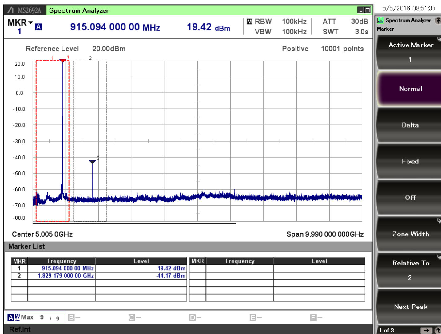
Figure 7.1. Typical Output Spectrum of the BRD4150B
