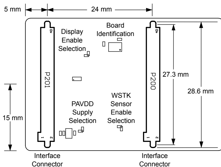
Figure 5.2. BRD4150B Bottom View
