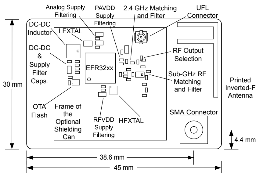
Figure 5.1. BRD4150B Top View
