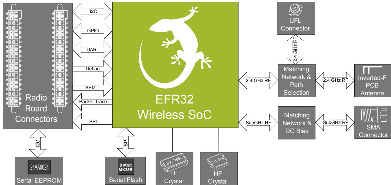
Figure 3.1. BRD4150B Block Diagram
