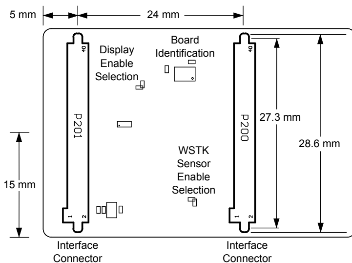
Figure 5.2. BRD4152A Bottom View
