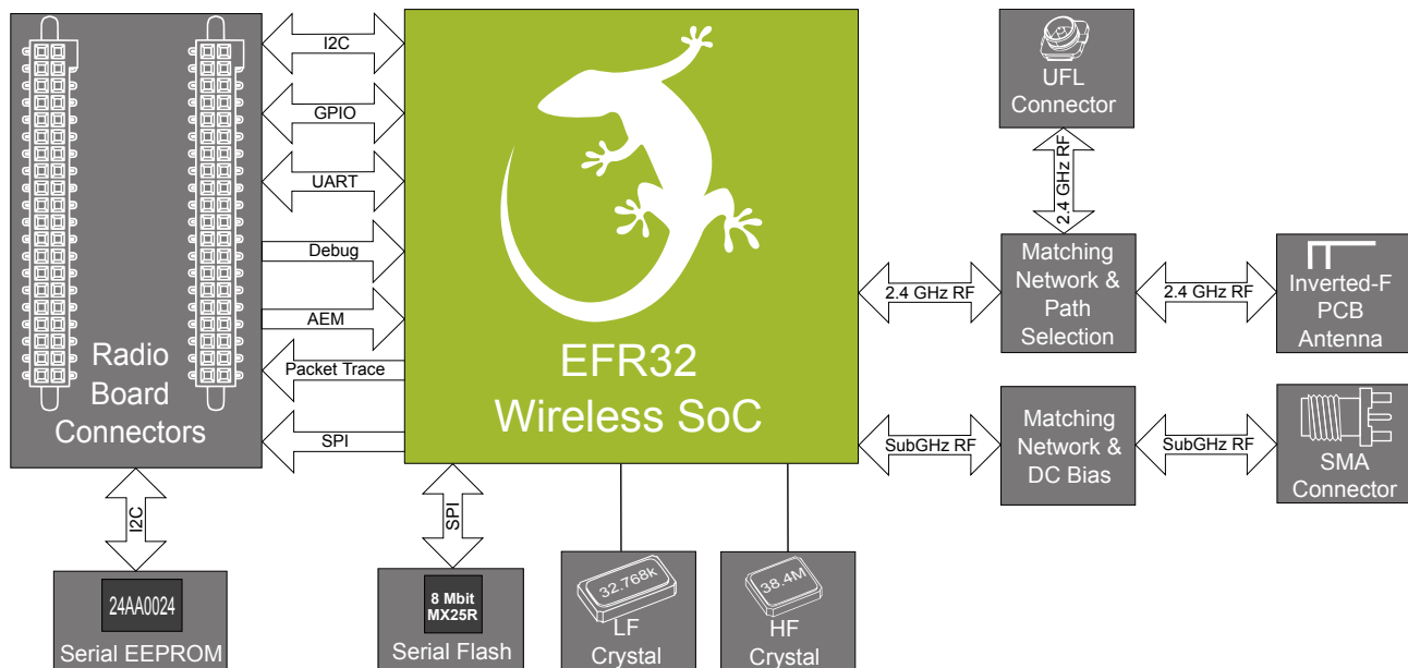
Figure 3.1. BRD4152A Block Diagram
