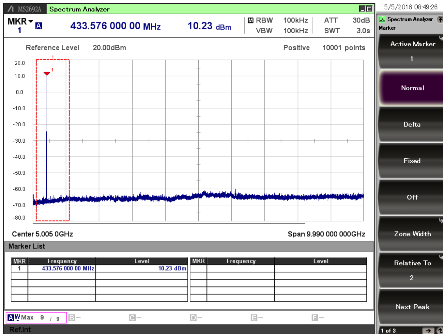
Figure 7.1. Typical Output Spectrum of the BRD4152A
