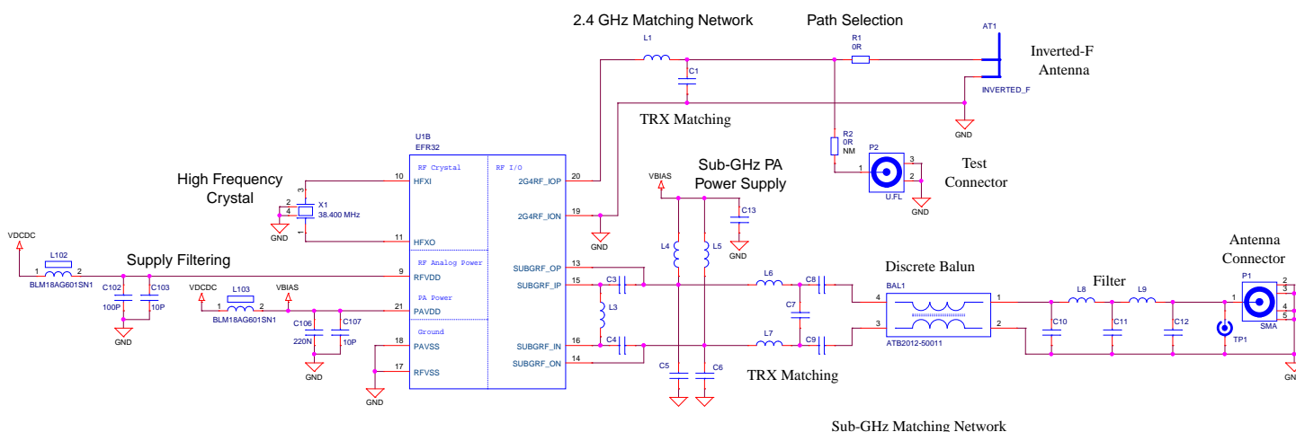
Figure 4.1. Schematic of the RF Section of the BRD4152A
