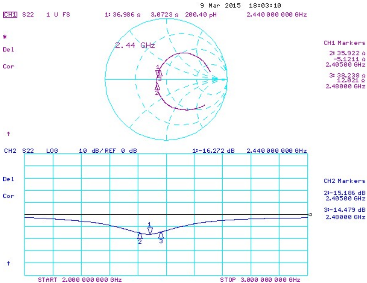
Figure 4.2. Impedance and Reflection of the Inverted-F Antenna of the BRD4152A
