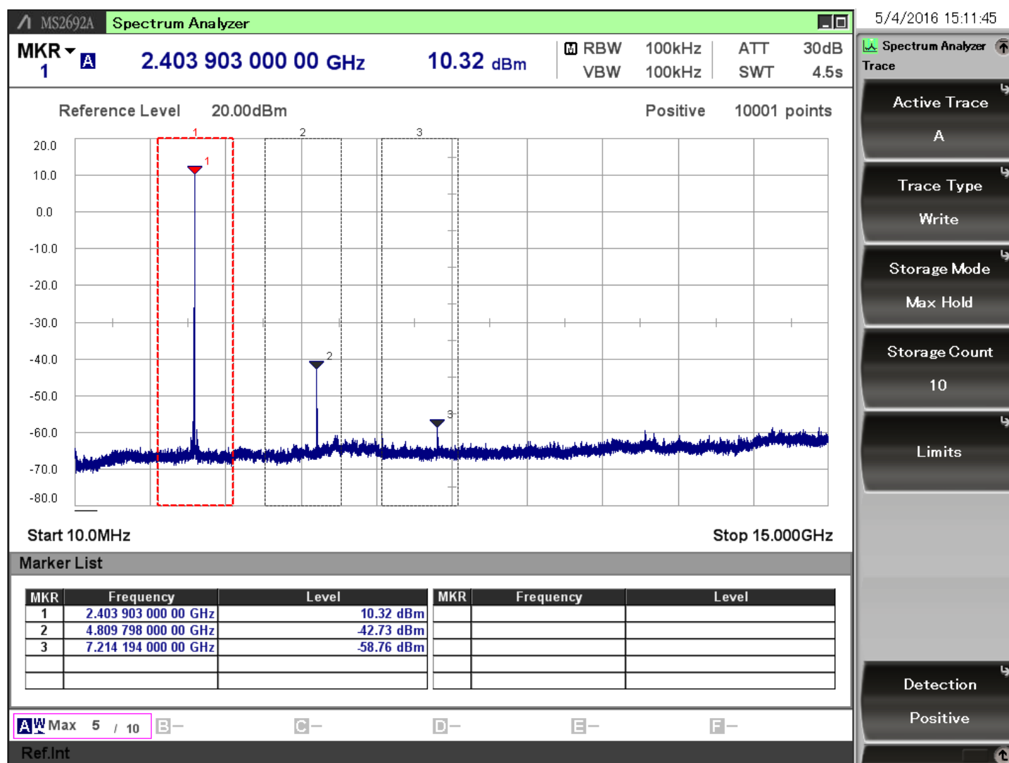
Figure 7.2. Typical Output Spectrum of the BRD4152A
