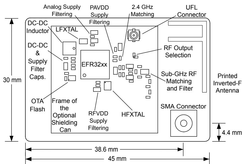
Figure 5.1. BRD4152A Top View
