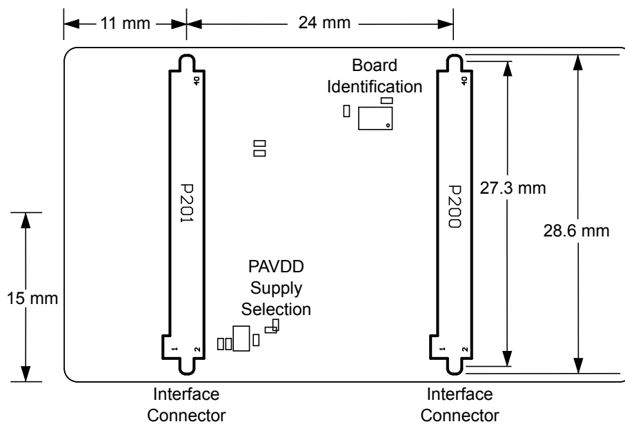
Figure 5.2. BRD4162A Bottom View
