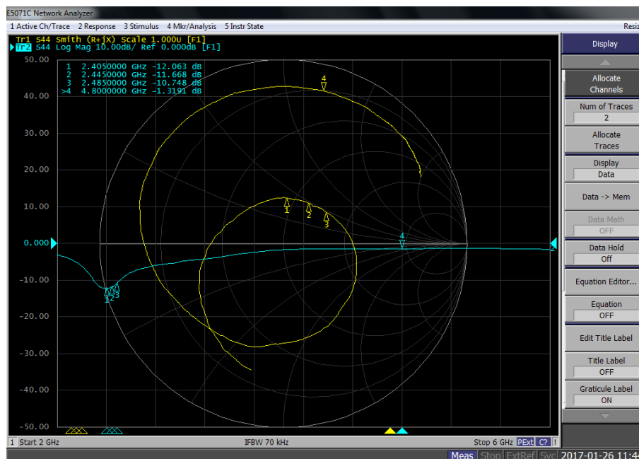
Figure 4.2. Impedance and Reflection of the Inverted-F Antenna of the BRD4162A Board Measured from the Matching Output
