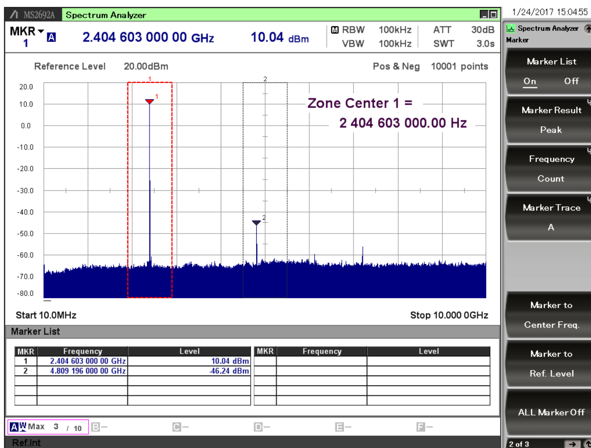
Figure 7.1. Typical Output Spectrum of the BRD4162A
