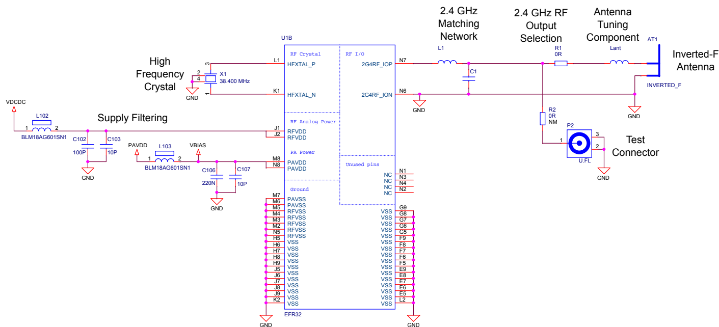
Figure 4.1. Schematic of the RF Section of the BRD4162A
