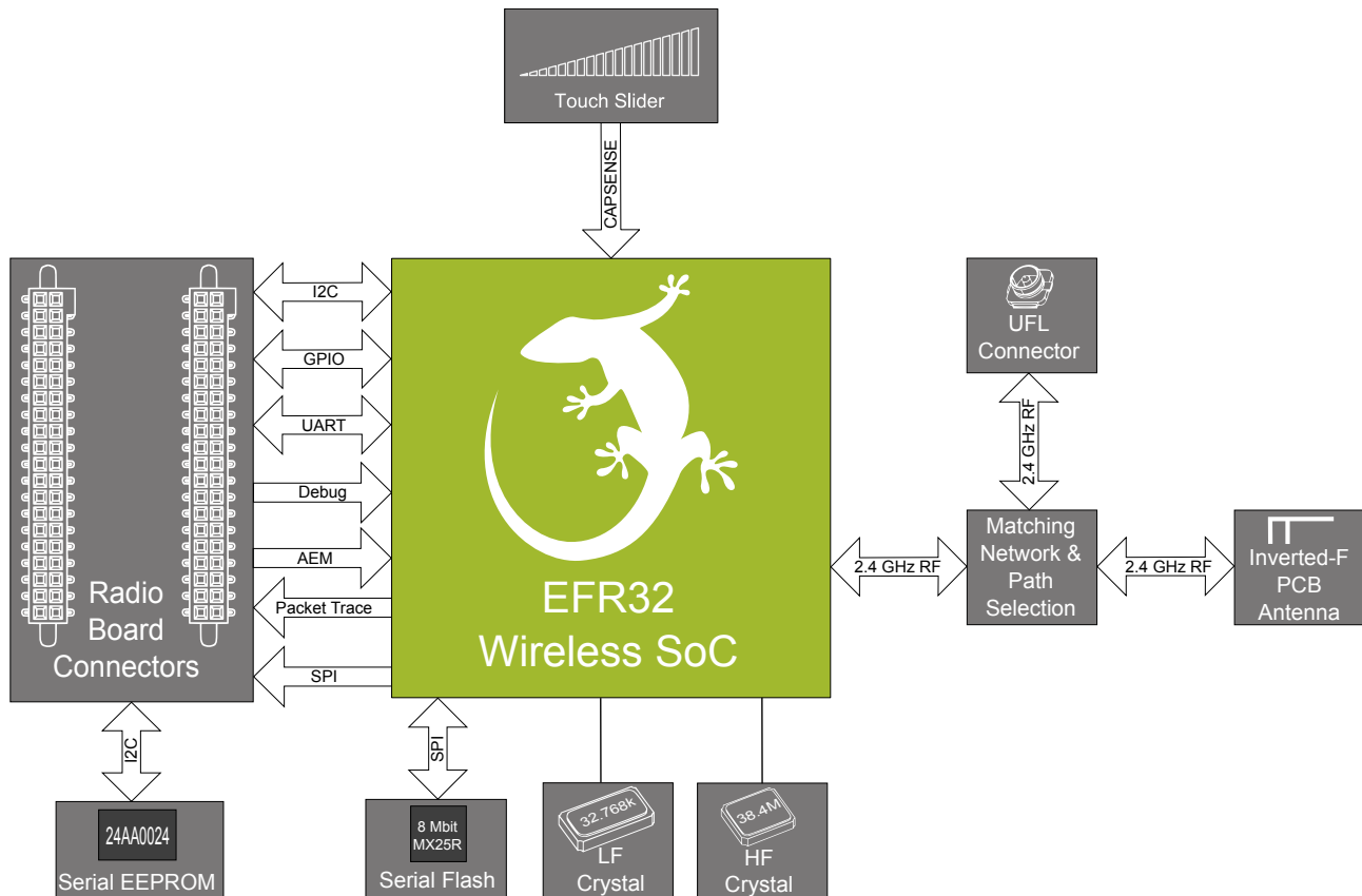
Figure 3.1. BRD4162A Block Diagram
