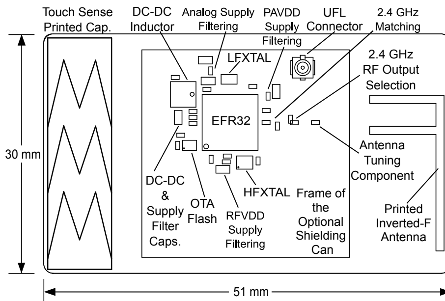
Figure 5.1. BRD4162A Top View
