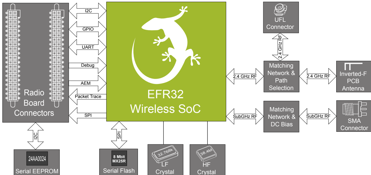
Figure 3.1. BRD4251A Block Diagram
