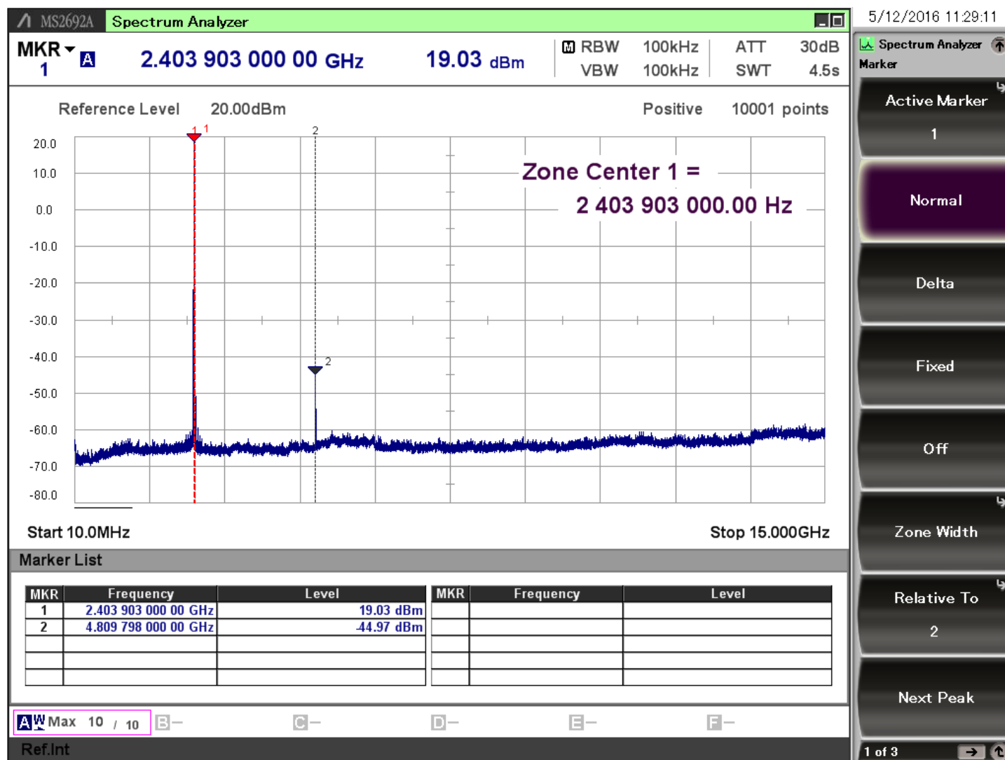
Figure 7.2. Typical Output Spectrum of the BRD4251A
