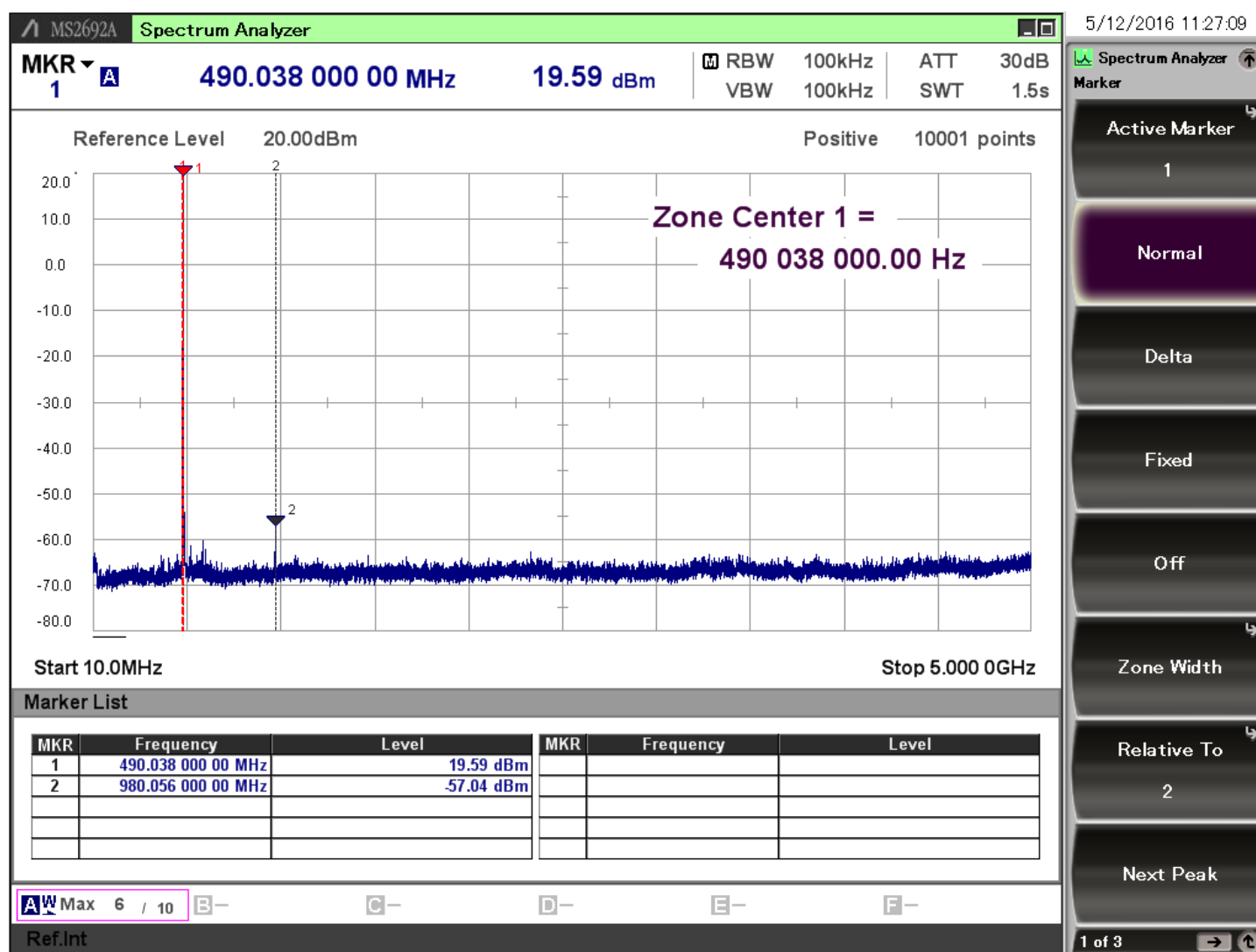
Figure 7.1. Typical Output Spectrum of the BRD4251A
