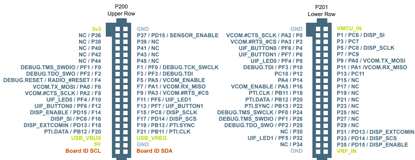
Figure 2.1. BRD4251A Radio Board Connector Pin Mapping
