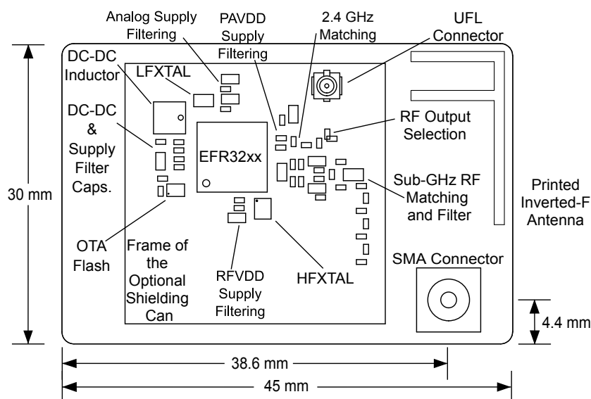
Figure 5.1. BRD4251A Top View
