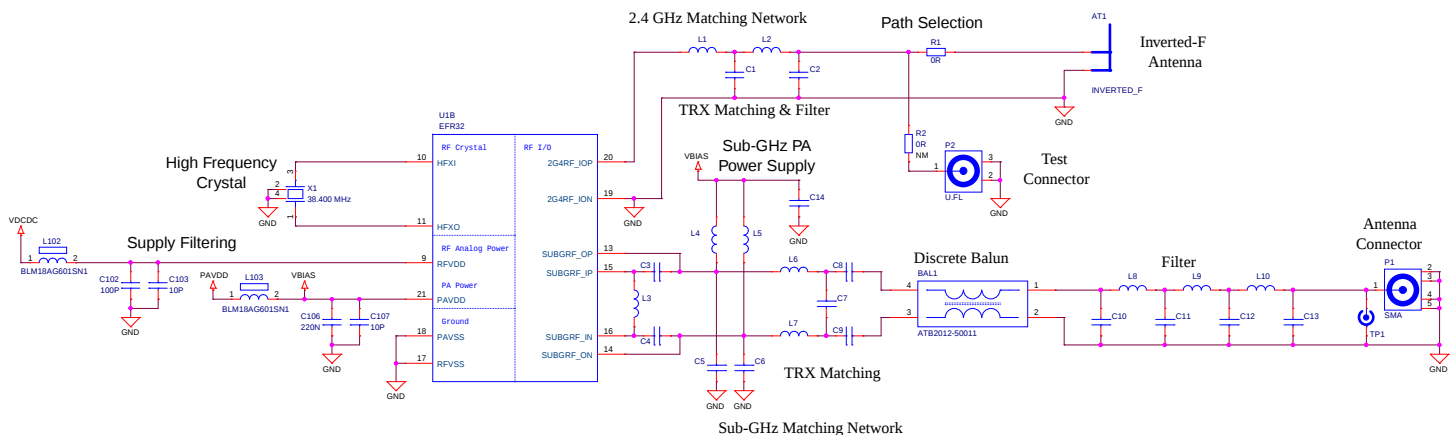
Figure 4.1. Schematic of the RF Section of the BRD4251A
