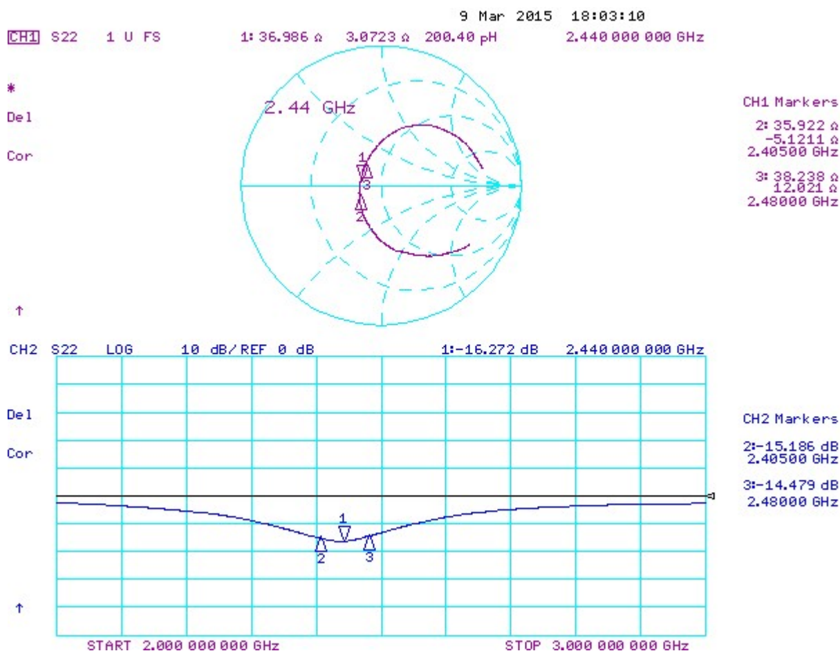
Figure 4.2. Impedance and Reflection of the Inverted-F Antenna of the BRD4251A
