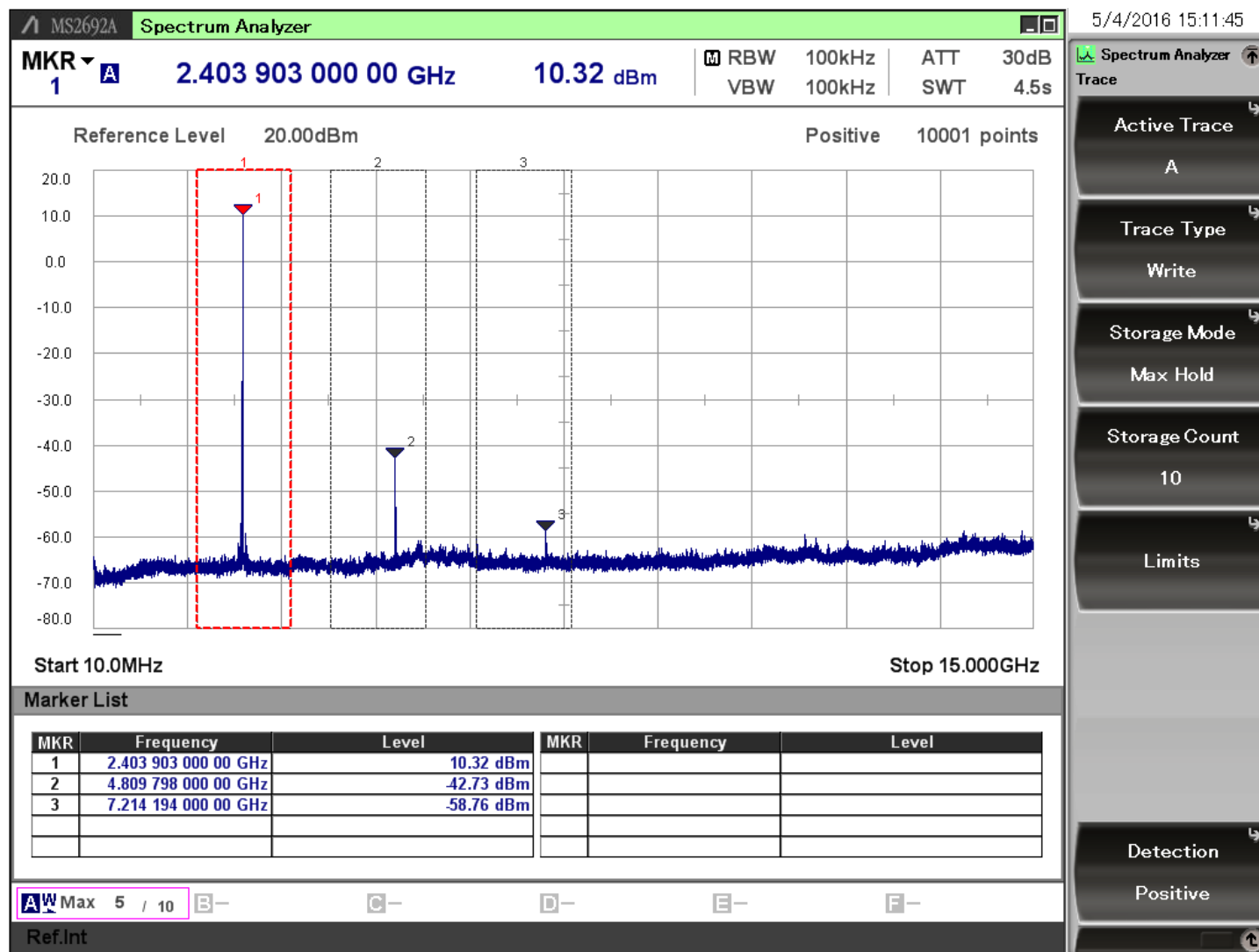
Figure 7.2. Typical Output Spectrum of the BRD4251B
