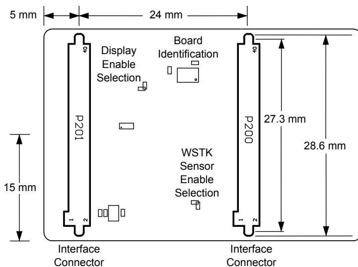
Figure 5.2. BRD4251B Bottom View
