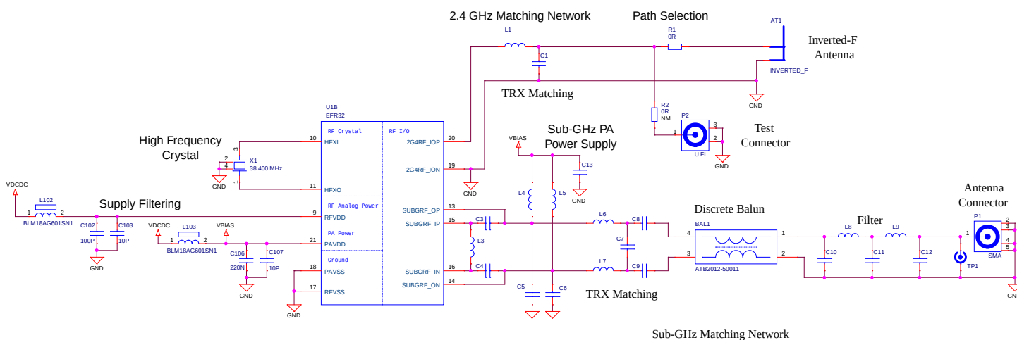
Figure 4.1. Schematic of the RF Section of the BRD4251B
