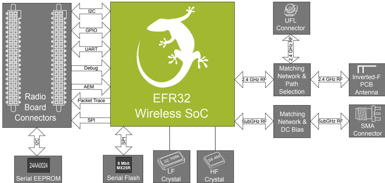
Figure 3.1. BRD4251B Block Diagram
