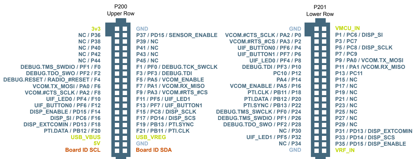
Figure 2.1. BRD4251B Radio Board Connector Pin Mapping
