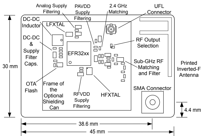
Figure 5.1. BRD4251B Top View
