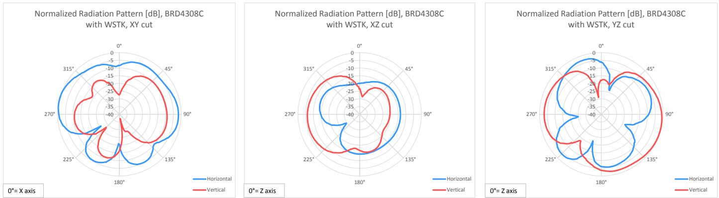
Figure 6.3. Normalized Antenna Pattern of the BRD4308C with the Wireless Starter Kit Mainboard
