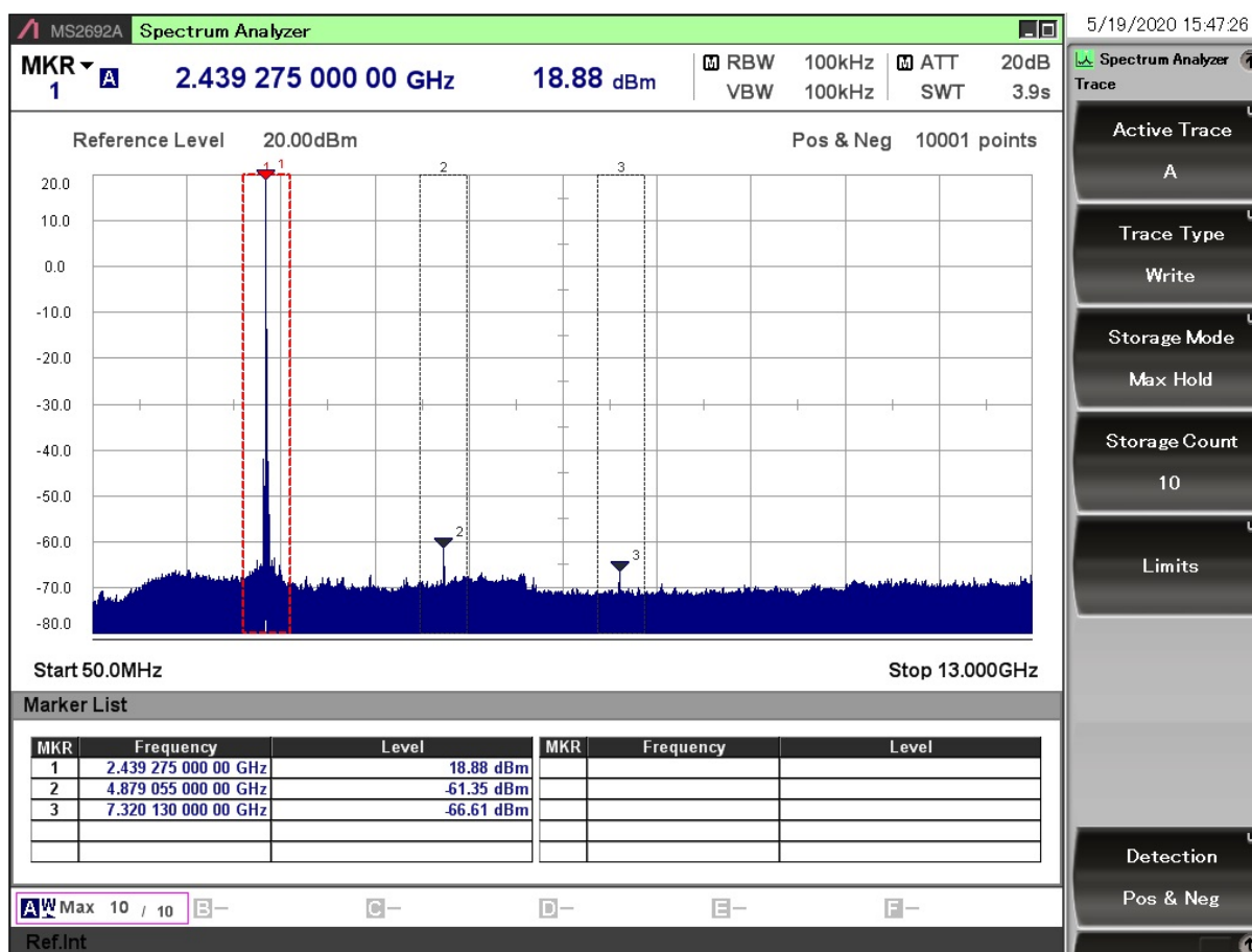
Figure 6.1. Typical Output Spectrum of the BRD4308C
