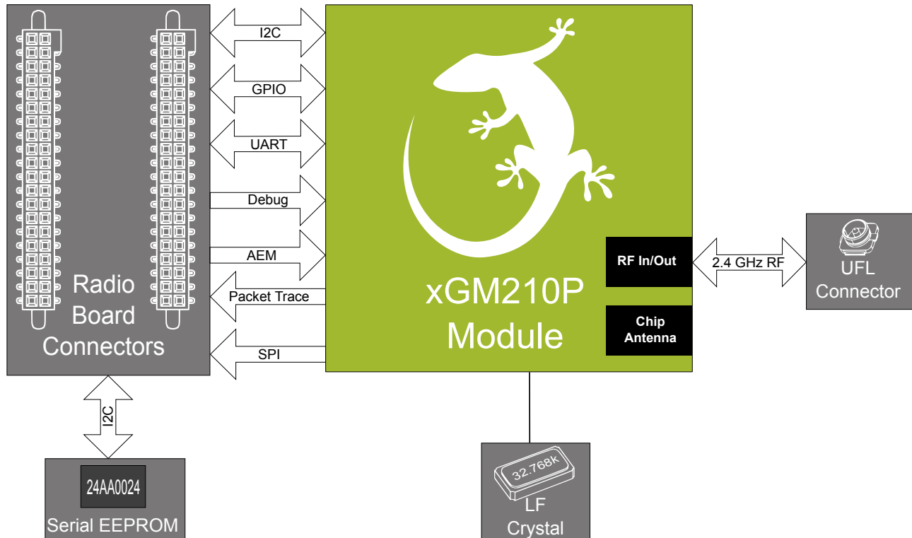
Figure 3.1. BRD4308C Block Diagram
