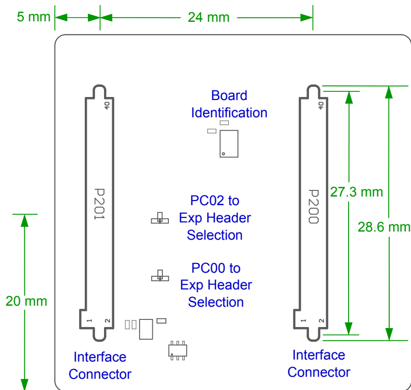
Figure 4.2. BRD4308C Bottom View
