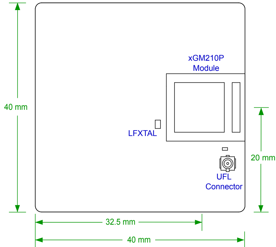
Figure 4.1. BRD4308C Top View
