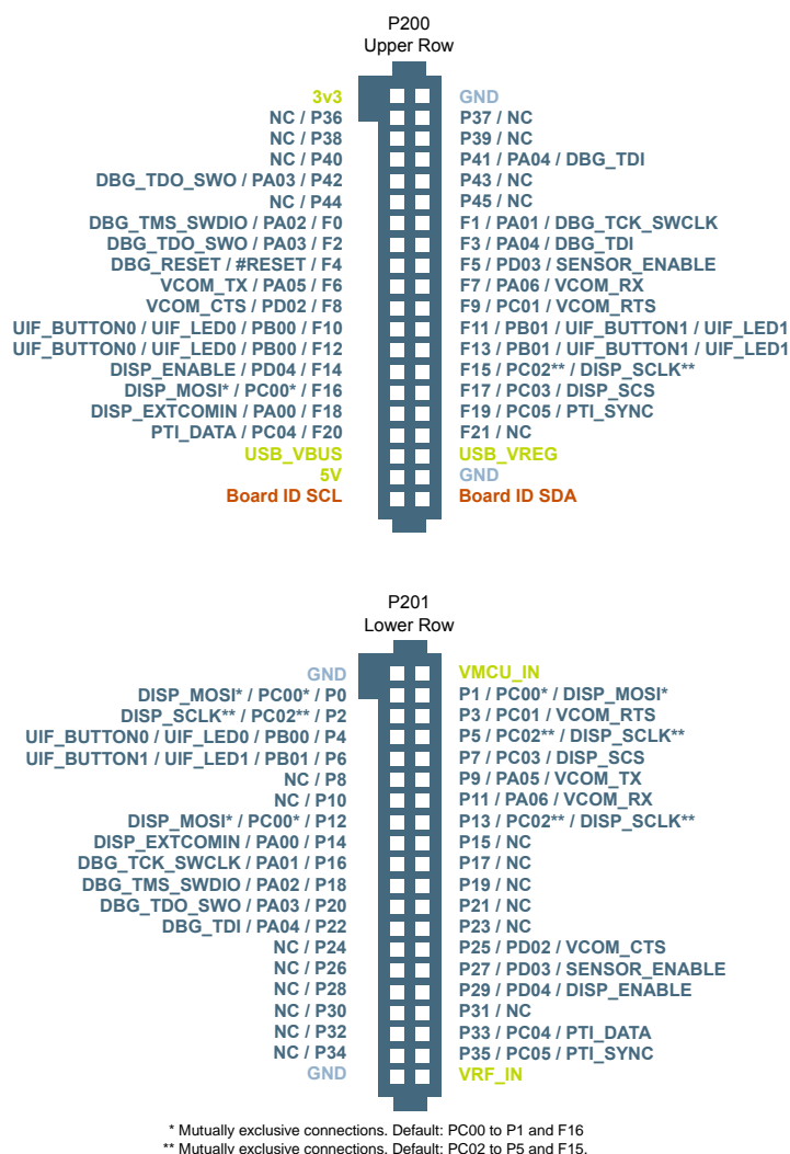
Figure 2.1. BRD4308C Radio Board Connector Pin Mapping
