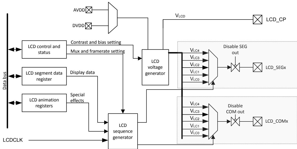
Figure 31.1. LCD Block Diagram
