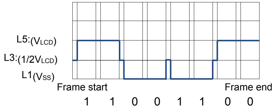
Figure 31.51. LCD Charge Redist - 1/2 Bias and Quadruplex Multiplexing - LCD.SEG0
