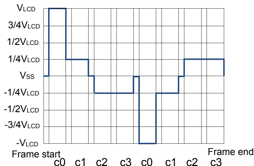
Figure 31.59. LCD Charge Redist - 1/4 Bias and Quadruplex Multiplexing - LCD.SEG0-LCD.COM0
