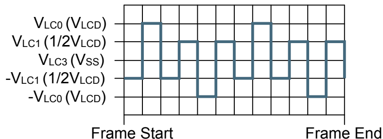
Figure 31.24. LCD 1/2 Bias and Triplex Multiplexing - LCD.SEG0-LCD.COM1
