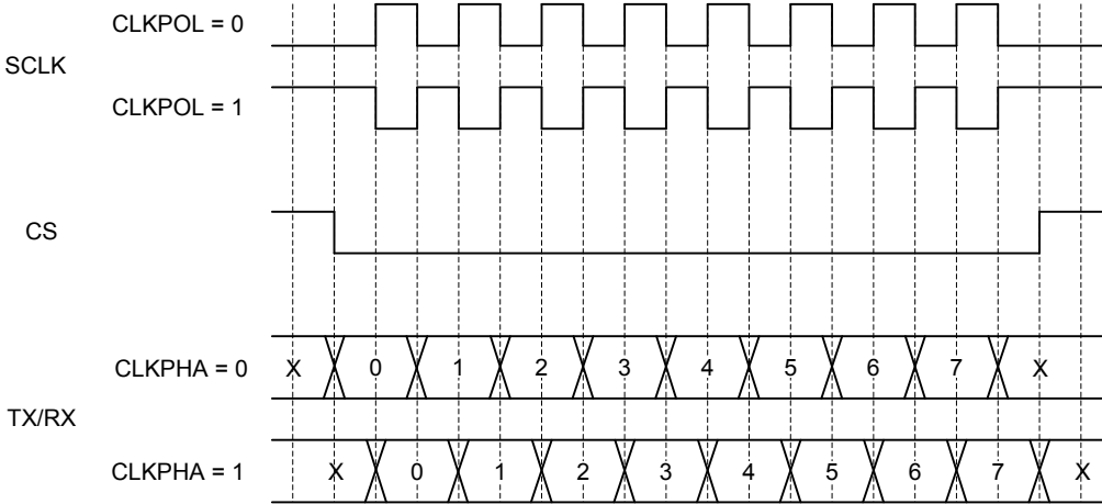
Figure 20.18. EUSART SPI Timing
