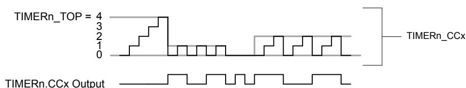
Figure 18.19. TIMER Up-count Frequency Generation Detail
