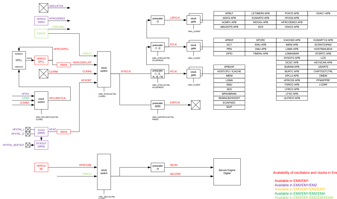
Figure 7.1. Bus Clocks
