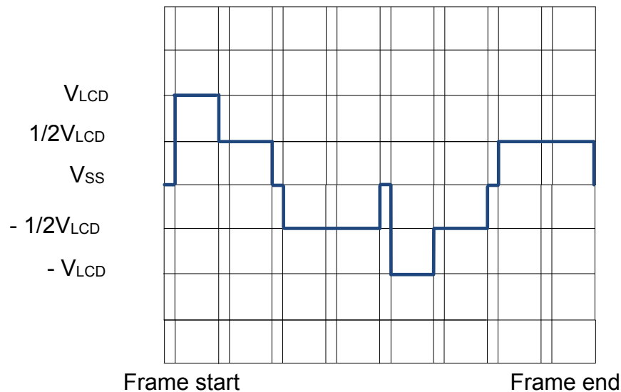
Figure 31.53. LCD Charge Redist - 1/2 Bias and Quadruplex Multiplexing - LCD.SEG0-LCD.COM0
