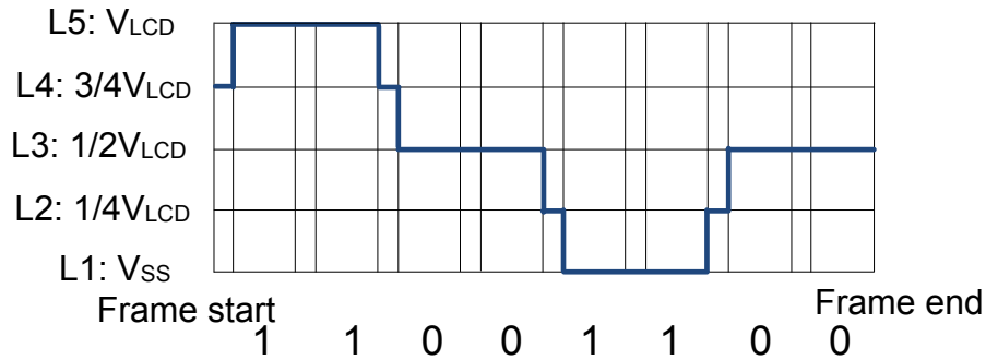
Figure 31.57. LCD Charge Redist - 1/4 Bias and Quadruplex Multiplexing - LCD.SEG0
