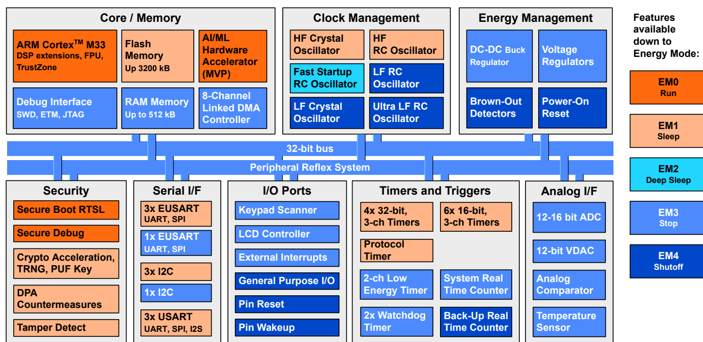
Figure 2.1. EFM32PG26 System-On-Chip Block Diagram
