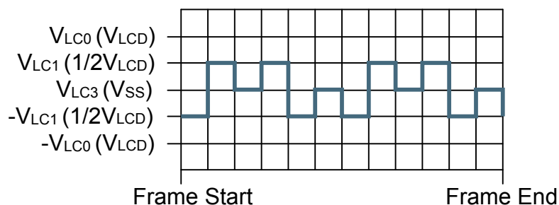
Figure 31.25. LCD 1/2 Bias and Triplex Multiplexing - LCD.SEG0-LCD.COM2
