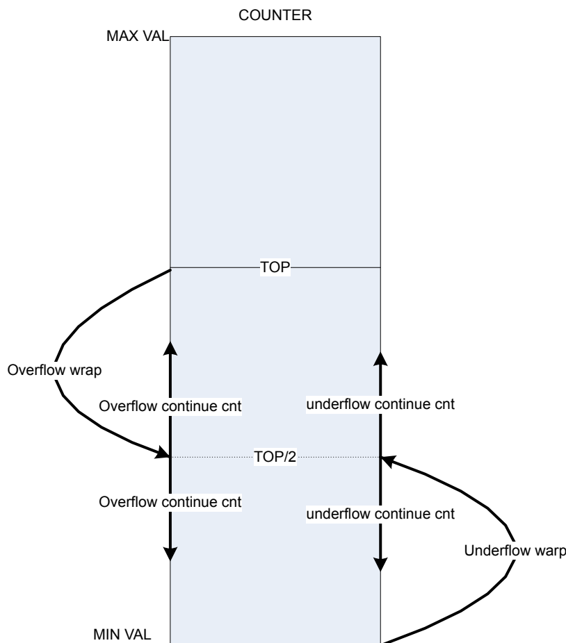
Figure 26.8. PCNT Hysteresis behavior of Counter
