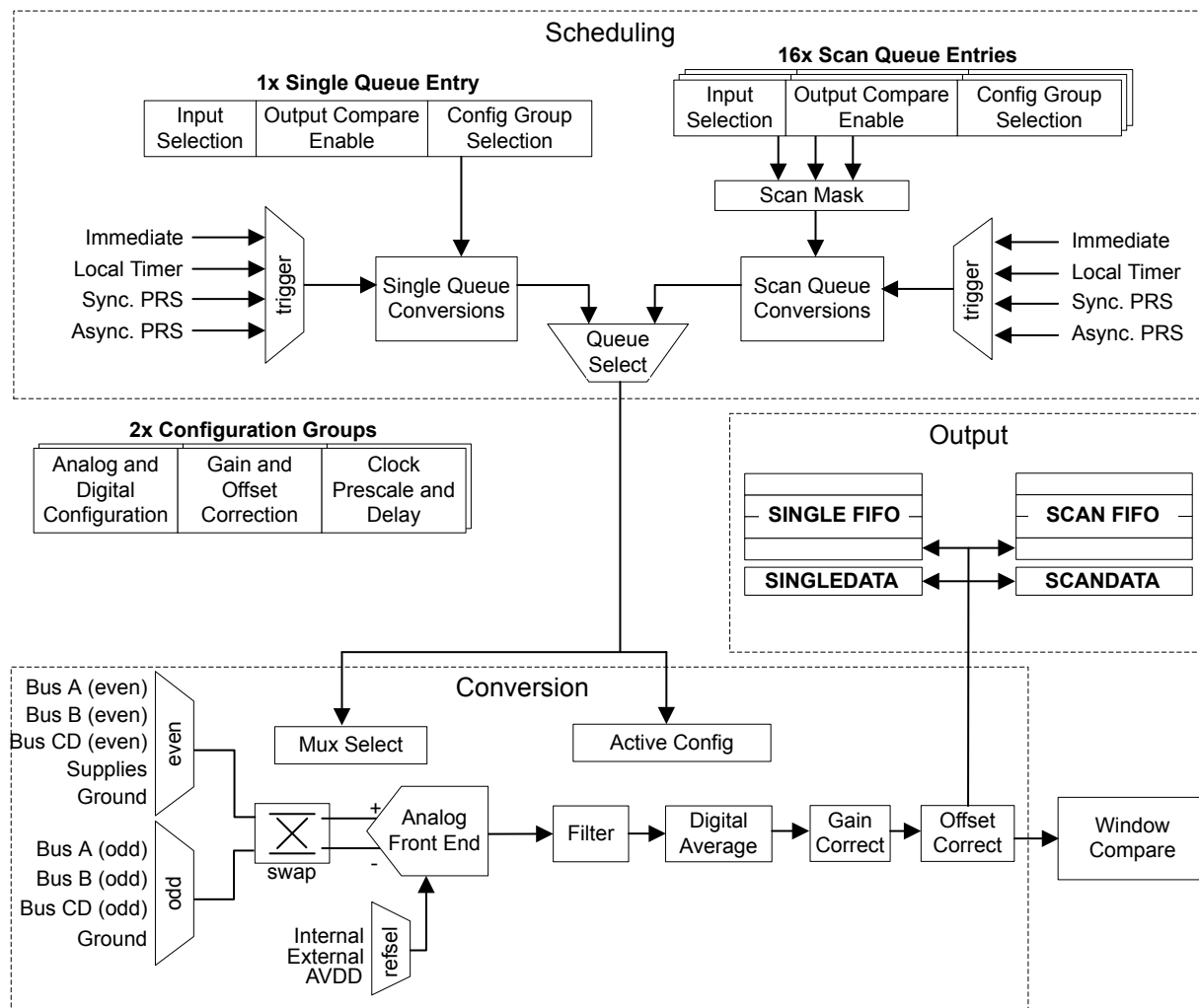
Figure 22.1. IADC Overview
