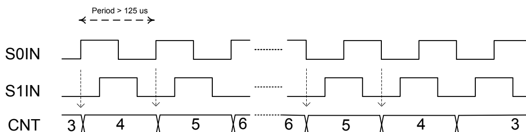
Figure 26.4. PCNT Oversampling Quadrature Decoder 1X Mode
