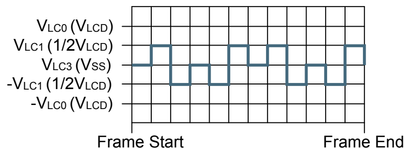
Figure 31.23. LCD 1/2 Bias and Triplex Multiplexing - LCD.SEG0-LCD.COM0
