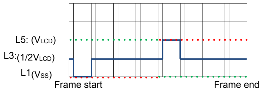
Figure 31.52. LCD Charge Redist - 1/2 Bias and Quadruplex Multiplexing - LCD.COM0
