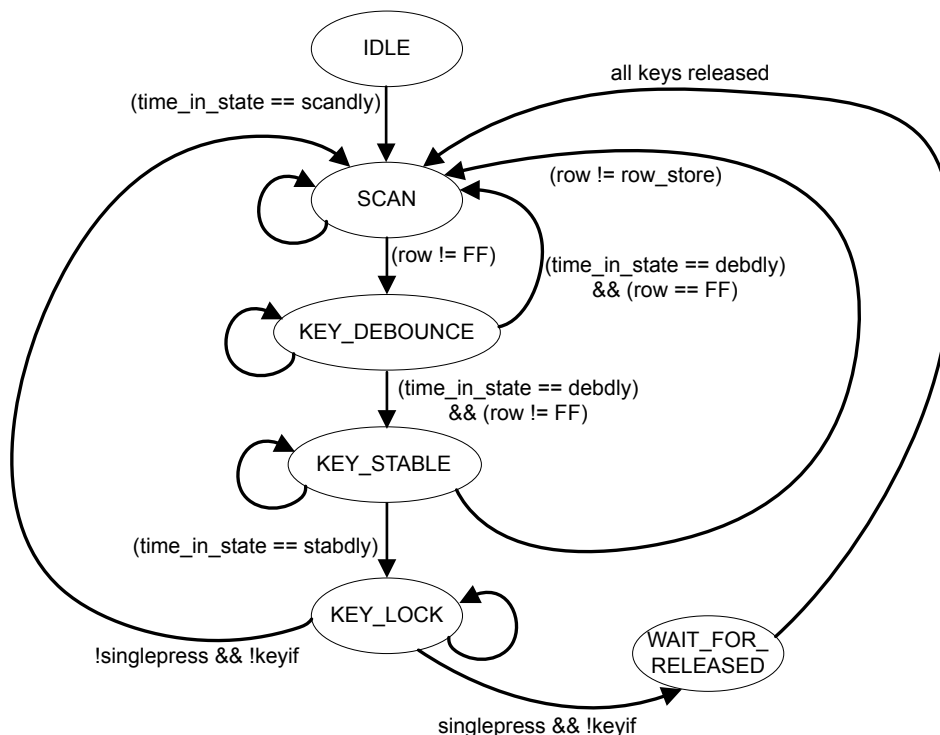
Figure 29.2. KEYSCAN State Machine
