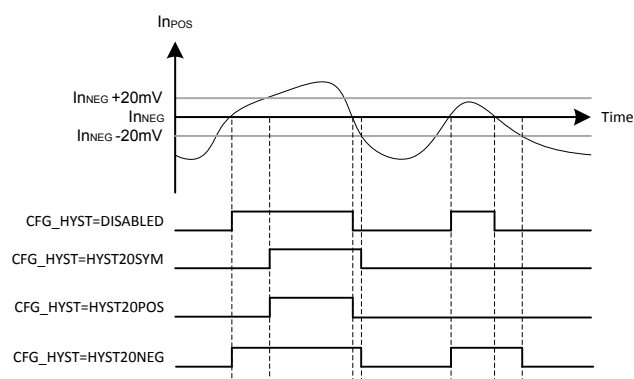
Figure 28.2. Hysteresis
