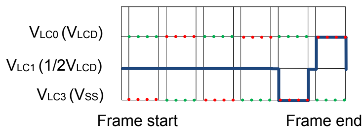
Figure 31.46. LCD Charge Redist - 1/2 Bias and Triplex Multiplexing - LCD.COM2
