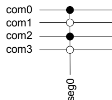
Figure 31.39. LCD 1/3 Bias and Quadruplex Multiplexing - LCD.SEG0 Connection
