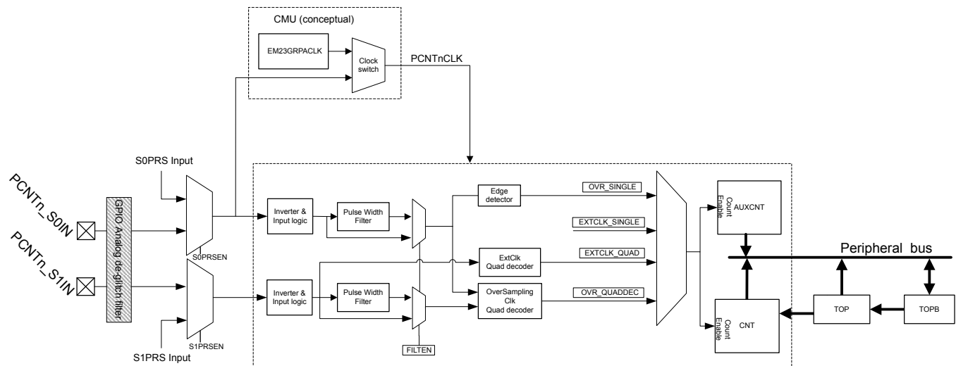
Figure 26.1. PCNT Overview
