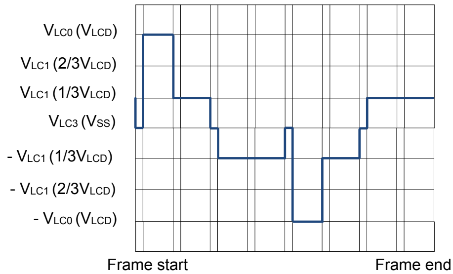
Figure 31.56. LCD Charge Redist - 1/3 Bias and Quadruplex Multiplexing - LCD.SEG0-LCD.COM0
