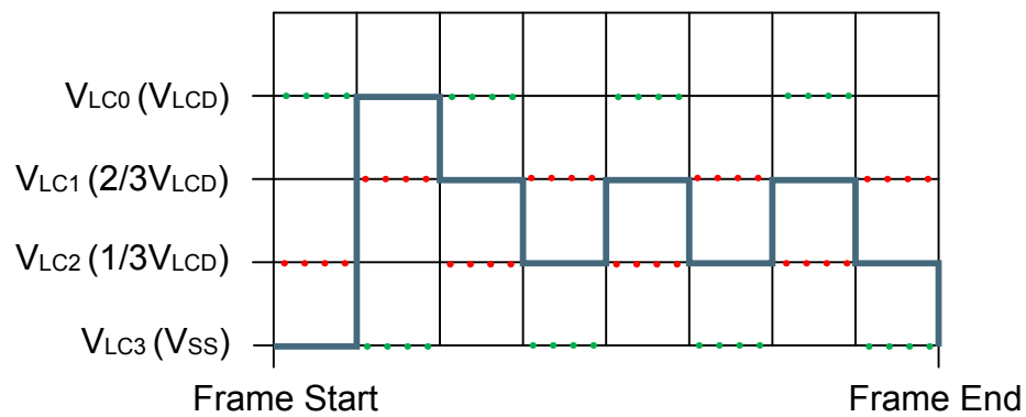
Figure 31.3. LCD Type A Waveform for LCD.COM0 in Quadruplex Multiplex Mode, 1/3 Bias
