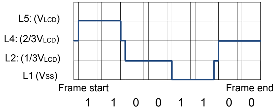
Figure 31.54. LCD Charge Redist - 1/3 Bias and Quadruplex Multiplexing - LCD.SEG0
