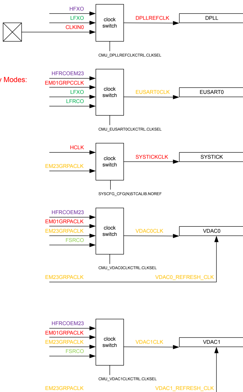
Figure 7.4. Mixed Frequency Peripheral Clocks
