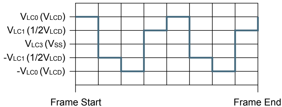
Figure 31.10. LCD 1/2 Bias and Duplex Multiplexing - LCD.SEG0-LCD.COM0
