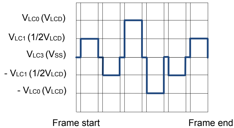
Figure 31.49. LCD Charge Redist - 1/2 Bias and Triplex Multiplexing - LCD.SEG0-LCD.COM1
