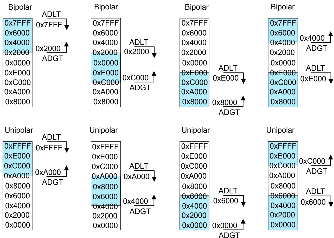
Figure 22.21. Window Comparison Examples
