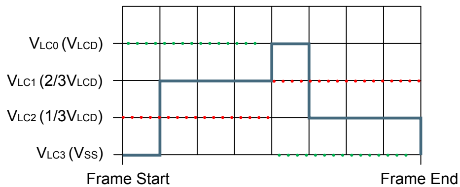
Figure 31.4. LCD Type B Waveform for LCD.COM0 in Quadruplex Multiplex Mode, 1/3 Bias
