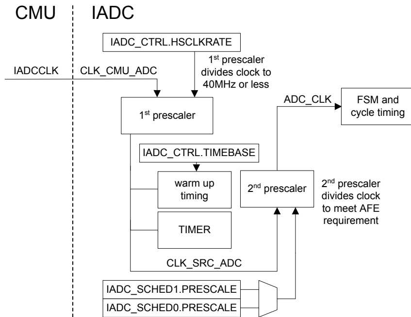
Figure 22.2. Clocking
