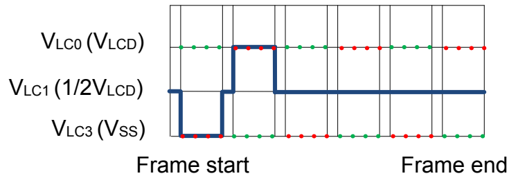
Figure 31.44. LCD Charge Redist - 1/2 Bias and Triplex Multiplexing - LCD.COM0
