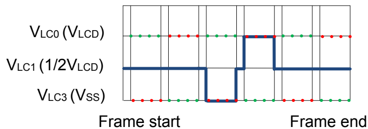
Figure 31.45. LCD Charge Redist - 1/2 Bias and Triplex Multiplexing - LCD.COM1
