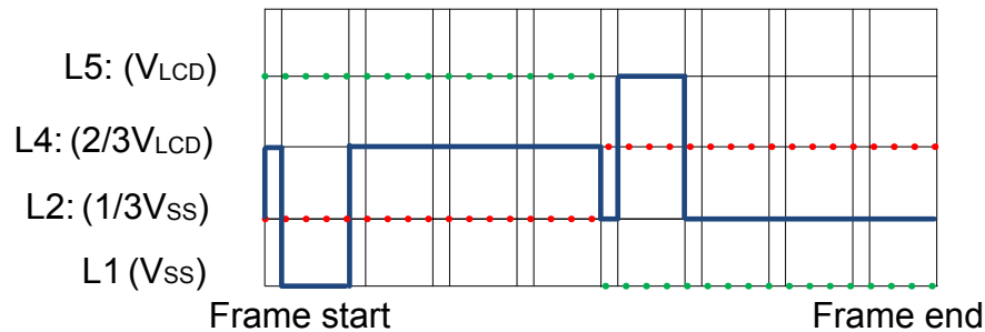
Figure 31.55. LCD Charge Redist - 1/3 Bias and Quadruplex Multiplexing - LCD.COM0
