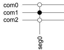
Figure 31.22. LCD 1/2 Bias and Triplex Multiplexing - LCD.SEG0 Connection
