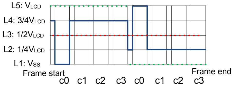
Figure 31.58. LCD Charge Redist - 1/4 Bias and Quadruplex Multiplexing - LCD.COM0
