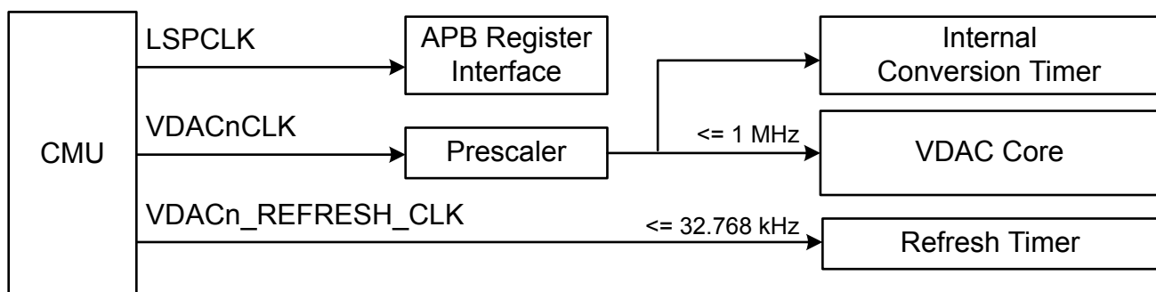
Figure 27.2. VDAC Block Clocks Diagram
