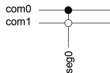
Figure 31.9. LCD 1/2 Bias and Duplex Multiplexing - LCD.SEG0 Connection
