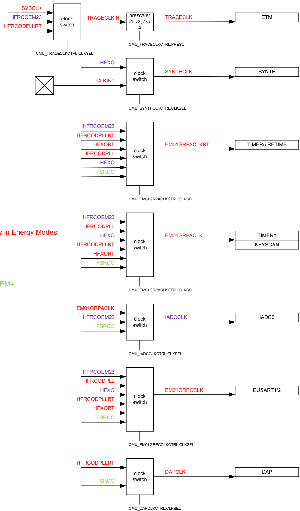
Figure 7.2. High Frequency Peripheral Clocks
