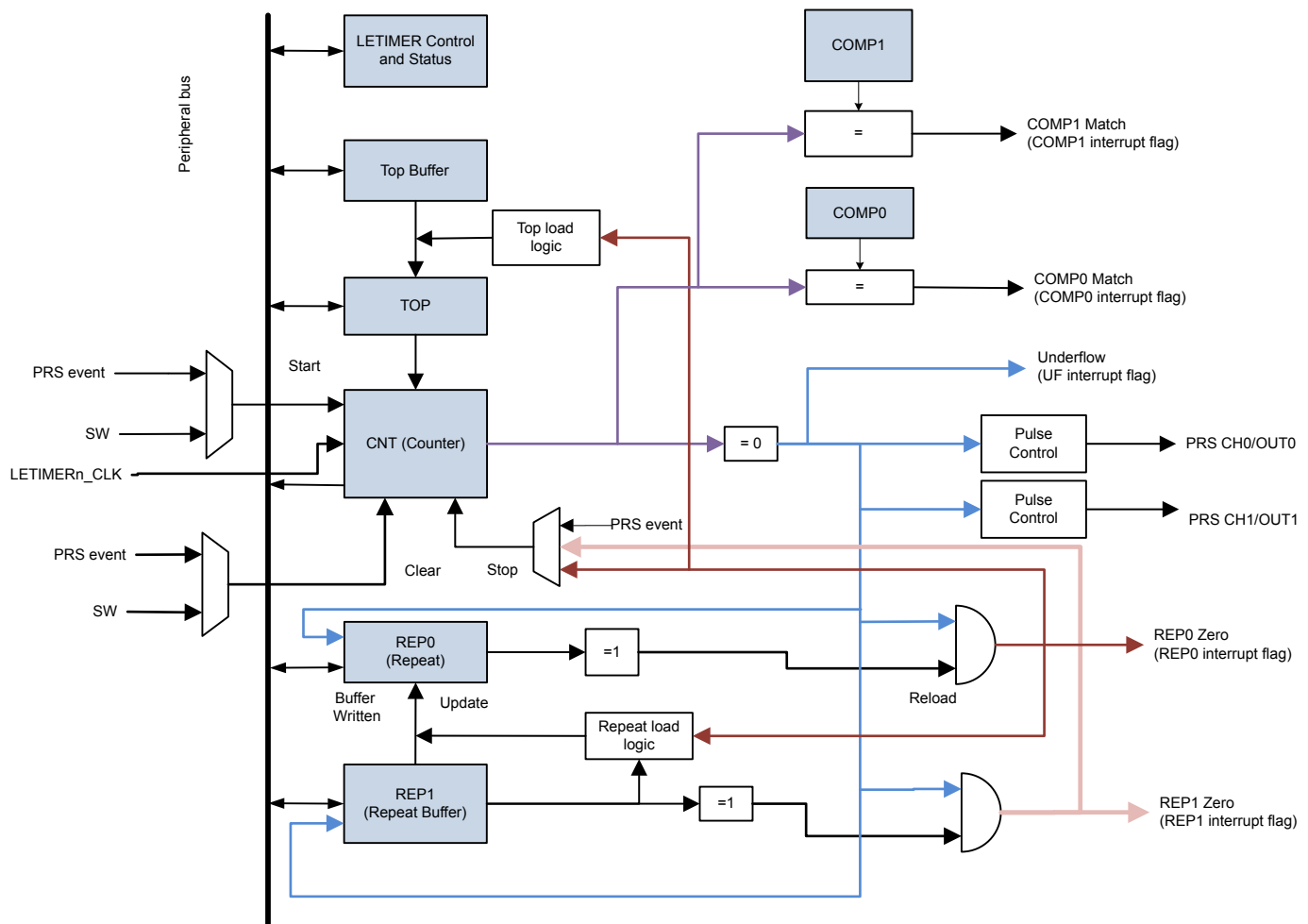
Figure 17.1. LETIMER Overview
