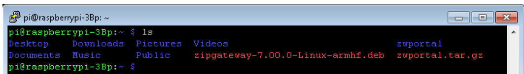
Figure 7: Z-Wave Source Copied to Target and Extracted in Folder zwportal
