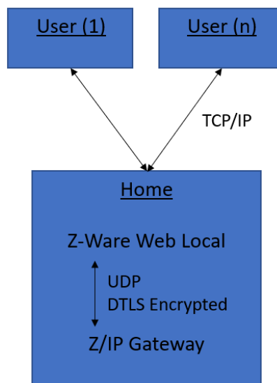
Figure 12: Setup with Z-Ware Local. No Support for Cloud.
