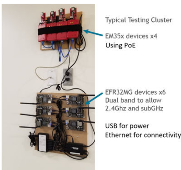
Figure 2.4. Large Network Test Setup
