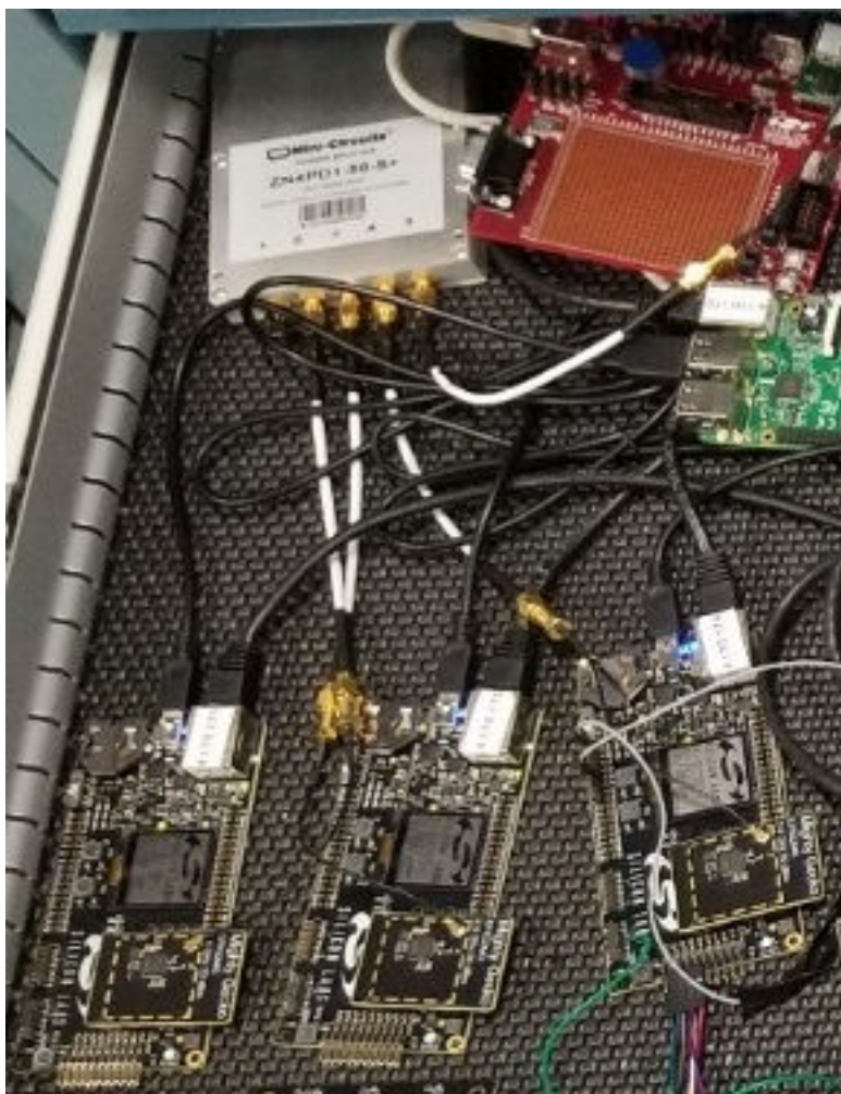
Figure 2.2. Multihop Test Network
