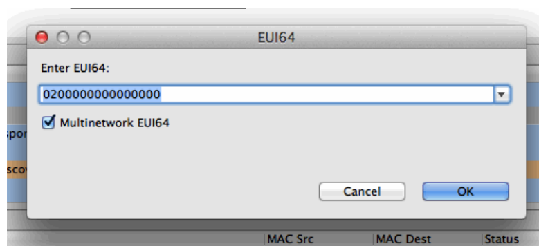
Figure 3.7. EUI64 Dialog
