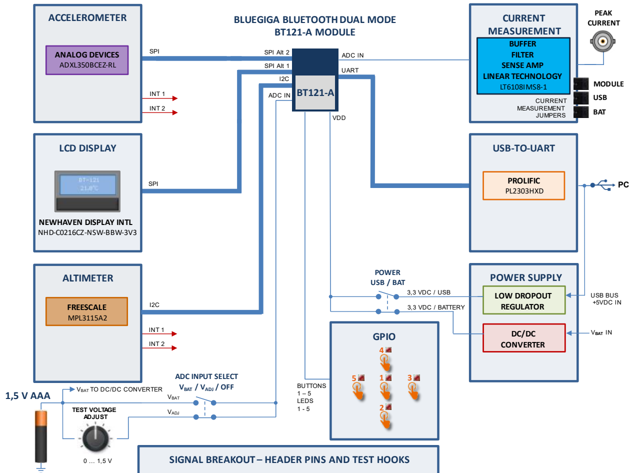
Figure 3: DKBT functional block diagram
