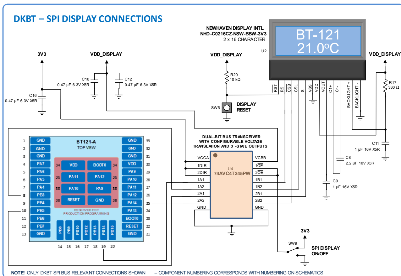
Figure 11: SPI display connections to BT121 in DKBT
