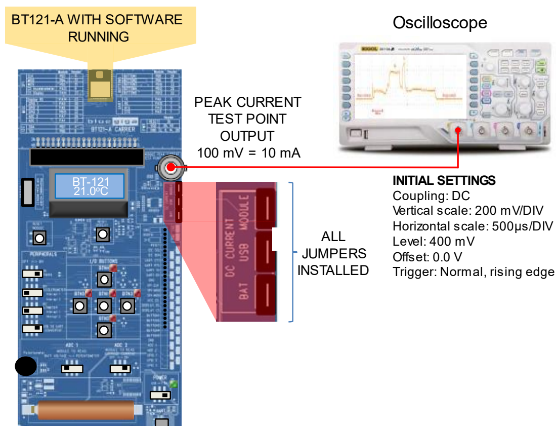
Figure 10: Peak current measurement using an oscilloscope.
