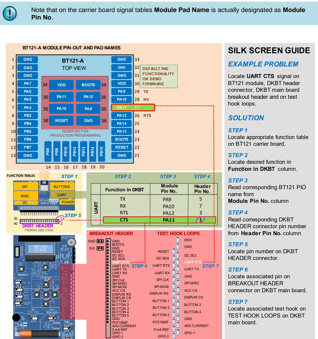
Figure 4: DKBT silk screen usage example.
