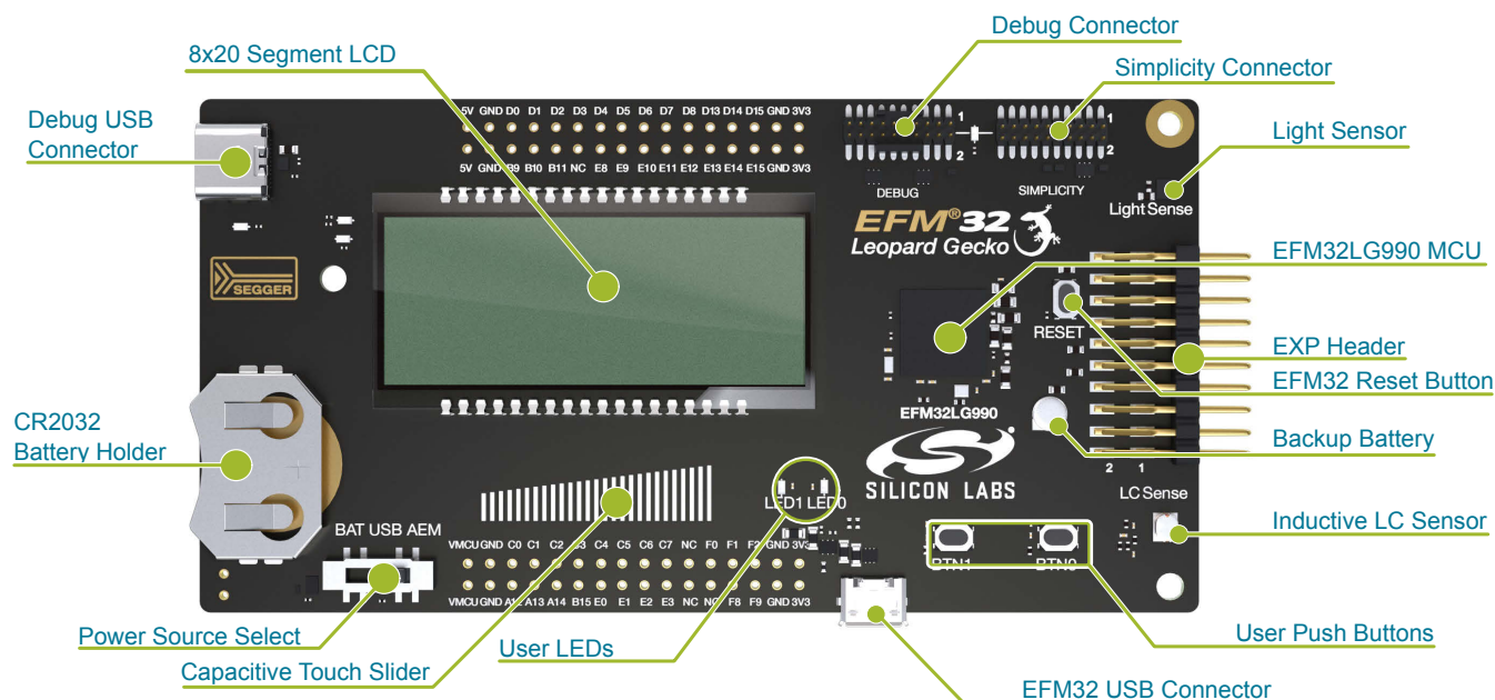
Figure 3.1. EFM32LG-STK3600A Hardware Layout
