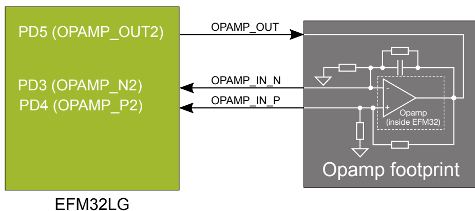
Figure 6.7. Opamp Footprint
