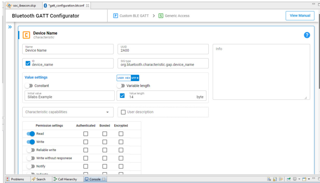
Figure 1.6: Settings Editor
