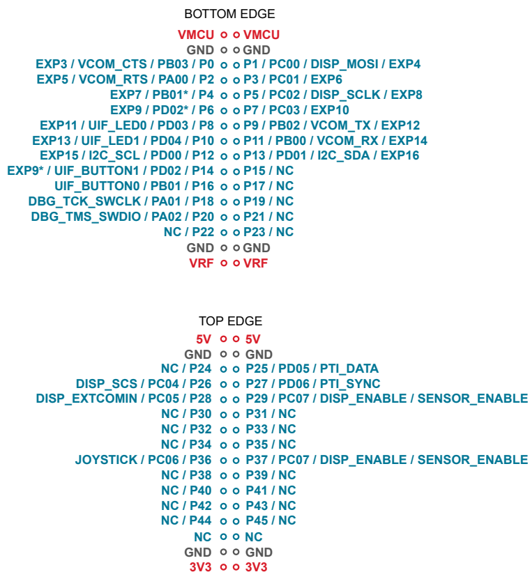
Figure 3.4. Wireless STK Mainboard (BRD4001A) Breakout Pad Pin Mapping
