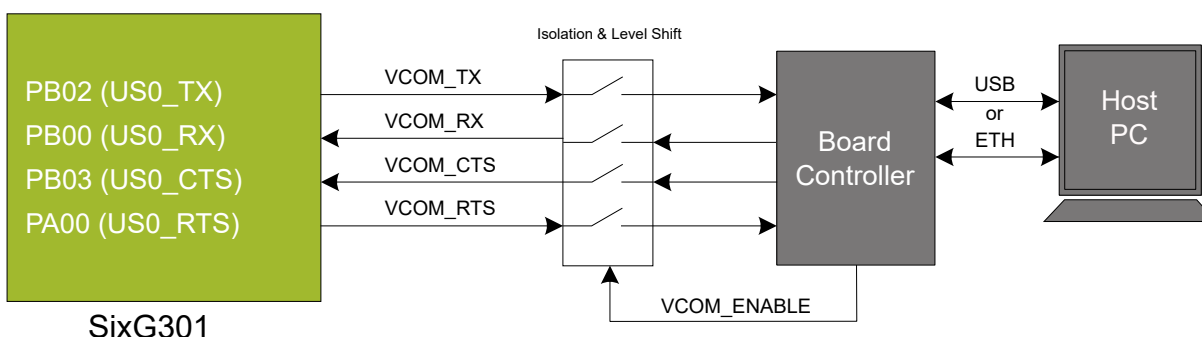
Figure 5.6. Virtual COM Port Interface
