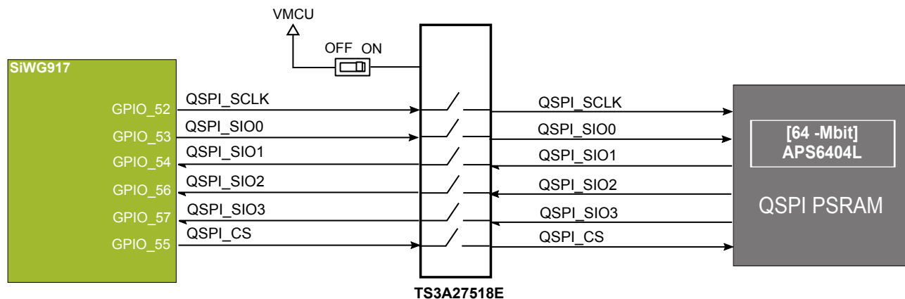
Figure 3.9. QSPI PSRAM
