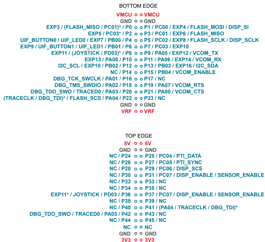
Figure 3.4. Wireless STK Mainboard (BRD4001A) Breakout Pad Pin Mapping
