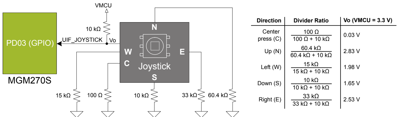
Figure 5.2. Joystick
