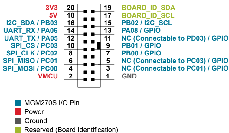
Figure 3.5. EXP Header
