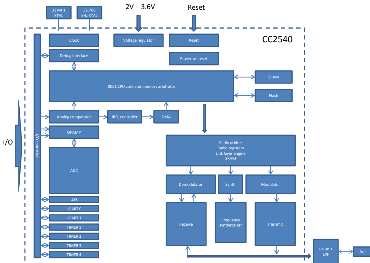
Figure 2: Simplified block diagram of BLE112
